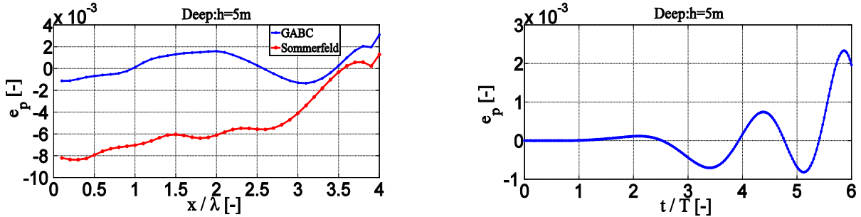
Figure 1: Spatial (left) and temporal (right) pointwise error in wave-only field
