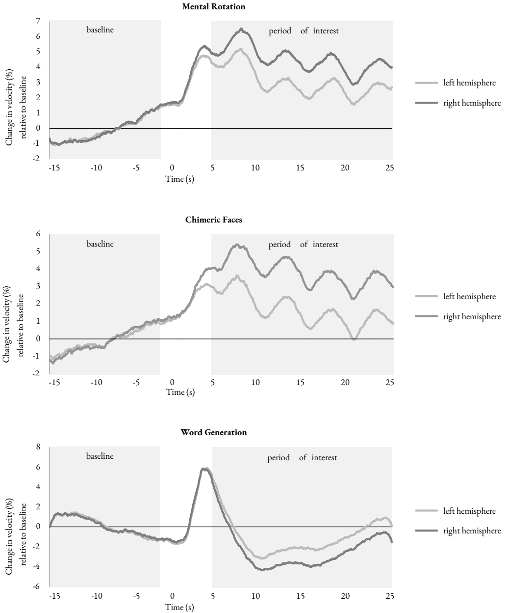
Figure A.5 Grand averages of fTCD measure by task.
