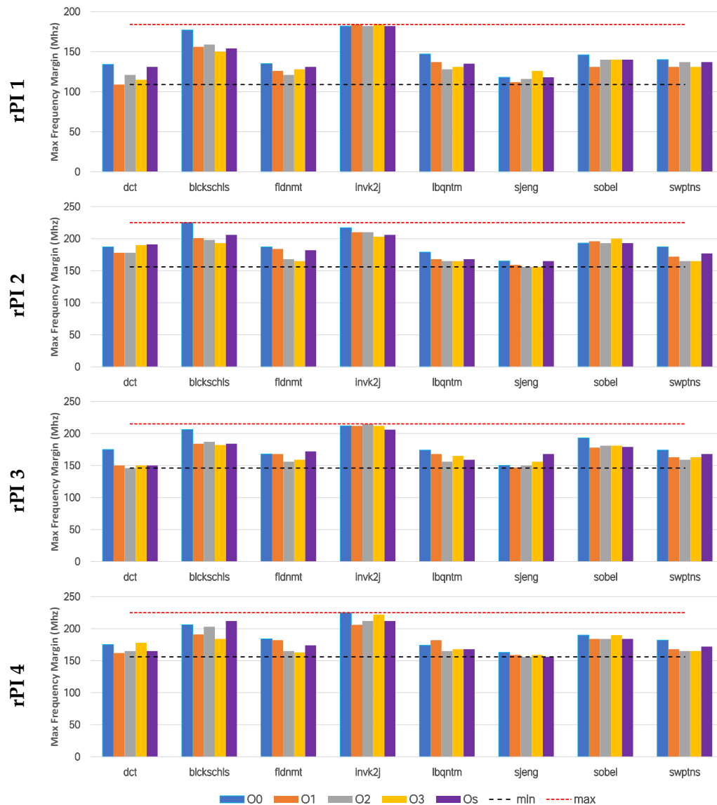
FIGURE 5.17: Evaluation of max_{fmargin} settings for 8 benchmarks (1000 runs each) in each raspberry PI; the higher the bar, the wider the exploitable frequency margin. The horizontal dotted lines show the maximum (red) and minimum (black) values of max_{fmargin} .
