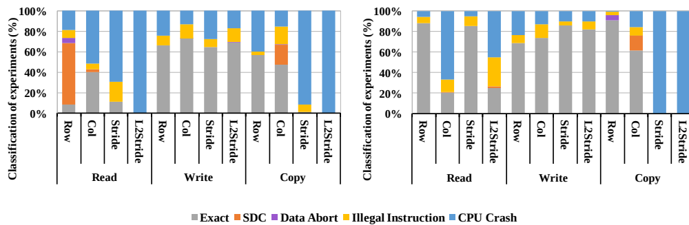
FIGURE 5.15: Experimental results of the Cache microkernels of Table 5.4 for unRel = (1.2V, 1430MHz) , when the hardware prefetcher is enabled (left) and disabled (right). The Y axis presents the classification of the experiments according to the effects of overclocked execution.
