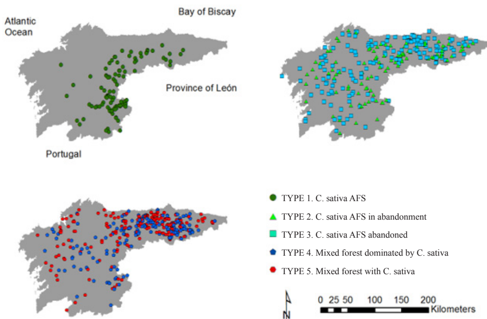
Figure 4. Spatial distribution of different types of Castanea sativa ecosystems in NW Spain. AFS=Agroforestry systems.
