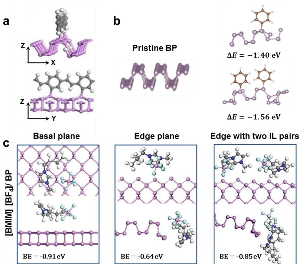
Figure 5: The DFT calculated structures of (a) Poly(phenylenevinylene) and BP along the zigzag direction viewing from the armchair direction on top and zigzag direction in the bottom [59] Copyright 2016, American Chemical Society (b) The pristine BP (left) along the armchair view and covalent bonding of aryl groups to BP (right) [60] Copyright 2016, Nature Publishing Group and (c) the structure of the strong chemisorption bonding of the [BMIM]-[BF 4 ] [62] on the BP basal plane, edge plane and the edge with two Ionic Liquids (IL) pairs, Copyright 2017, Wiley- Blackwell.
