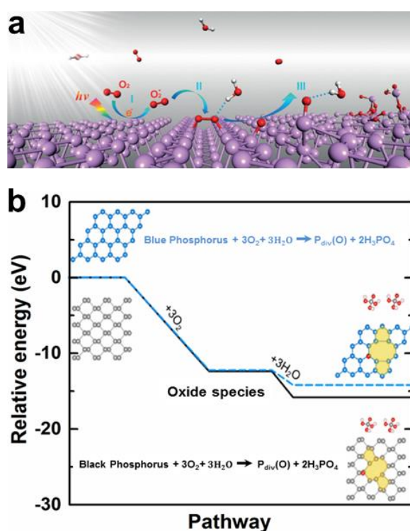
Figure 1: Schematic representations show: (a) a three-step process of BP degradation initiated by photo-oxidation. [28] Copyright 2016, Wiley- Blackwell (b) influence of O_2 and H_2O on black and blue phosphorene with respect to relative energy. [32] Image adapted from 2016, Institute of Physics Science Publishing.
