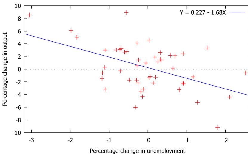
Fig. 2. Model-generated Okun’s curve. OLS estimation of the relationship between the percentage change in output and the percentage change in unemployment. R^2 = 0.1204 . The H_0 : “the estimated coefficient is not significantly different from zero” is rejected at the 1%.
