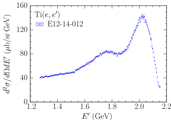
FIG. 3. Double-differential cross section for the \text{Ti}(e, e') process measured at beam energy of 2.222 GeV and fixed scattering angle of 15.541^\circ . The inner and outer uncertainty bars correspond to statistical and total uncertainties, respectively. The maximum uncertainties in the full kinematical range are provided.
