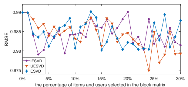
FIGURE 11: RMSE of the proposed methods on MU ( 401 \times 3952 )
