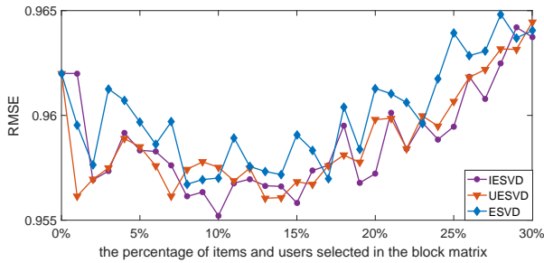
FIGURE 12: RMSE of the proposed methods on NI ( 6800 \times 500 )
