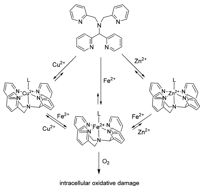
Scheme 1. Overview of the Coordination Chemistry of N4Py in Tumor Cells
