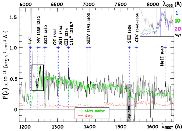
Figure 2. The FORS spectrum is shown with the main spectral features reported at the systemic redshift (blue crosses). In particular, the P-Cygni N \nu\lambda 1240, [C II]* \lambda 1335.71, [S IV] \lambda 1393, 1402, and the He II \lambda 1640 lines are highlighted with thick lines. The N \nu\lambda 1240 region (square) is zoomed and shown in the top-right inset (black line), in which three Starburst99 stellar models of 1, 10, and 20 Myr are superimposed to the spectrum (coloured lines).
