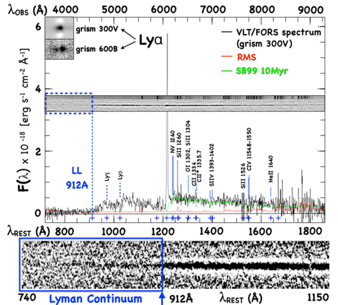
Figure 1. The FORS spectrum at resolution \text{dv} \simeq 580 \text{ km s}^{-1} (grism 300V) of Ion3 is shown along with the most relevant ultraviolet lines. In the top-left insets the Ly \alpha spectra at resolution \text{dv} \simeq 300(580) \text{ km s}^{-1} obtained with the grism 600B(300V) are shown. The two-dimensional signal to noise and sky spectra are shown in the middle of the figure, in which the wavelength coverage up to 9300 \text{ \AA} is well sampled, despite the fringing pattern at \lambda > 7800 \text{ \AA} typical of the E2V blue-optimized CCD. In the bottom the emerging LyC with \text{S/N} > 10 is clearly detected.
