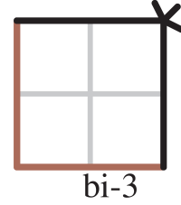
Fig. 17: Continuity properties of the surface cap. G^1 continuity for black edges, C^1 continuity for grey edges, C^0 continuity for brown edges. Taken from [3].
