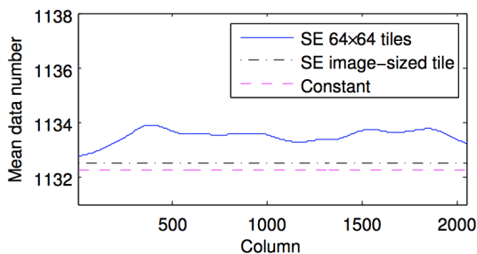
Fig. 5: Difference in background estimation for SExtractor and MTOObjects [10]
