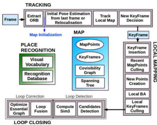
Fig. 4. Overview over the complete ORB-SLAM System.
