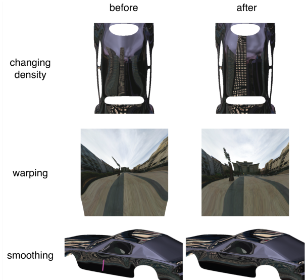
Fig. 19: Examples of reflection line optimization. Taken from [7].
