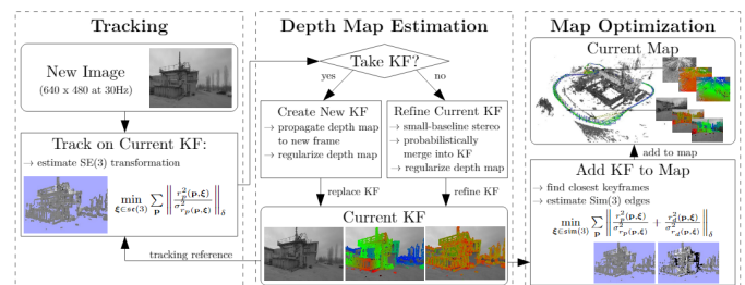
Fig. 6. Overview of LSD-SLAM algorithm.
