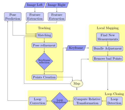
Fig. 5. Overview of S-PTAM process.
