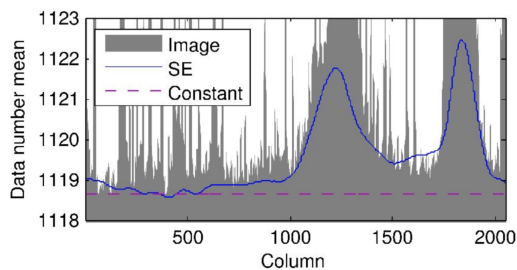
Fig. 4: Difference in background estimation for SExtractor and MTOObjects for a single image [8].
