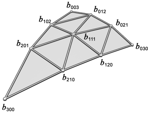
Fig. 4: The control points of the geometry. Vertex coefficients: b_{300} , b_{030} , b_{003} . Tangent coefficients: b_{210} , b_{120} , b_{201} , b_{021} , b_{102} , b_{012} . Center coefficient: b_{111} . Taken from [8].
