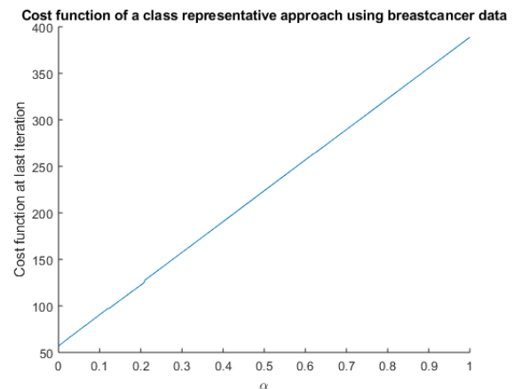
Fig. 10: Cost function of class representative GLVQ on breast cancer data
