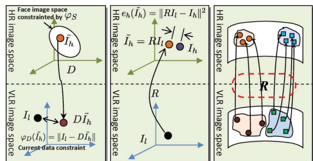
Fig. 5: Comparison of error calculation methods for human-based recognition. Left is the error calculation of existing approaches. The middle is the error calculation of the proposed approach. The right is the machine-based recognition approach. [13]
