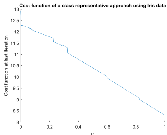
Fig. 2: Cost function of class representative GLVQ on iris data.
