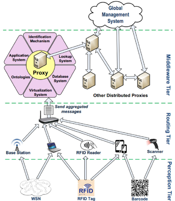
Fig. 4. Overall architecture of GGIoT.
