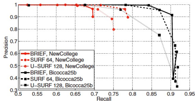
Fig. 7. Precision-recall curve of using BRIEF, SURF, and U-SURF on two datasets [7]
