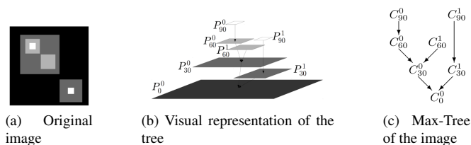
Fig. 2: Image and visual representation of its Max-Tree. Taken from [9]
