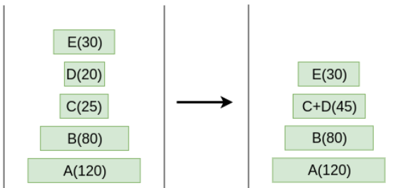
Figure 5: Breaking the invariant
