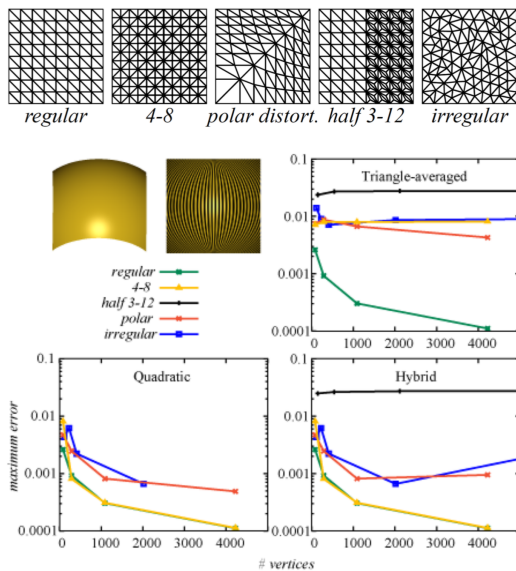
Fig. 22: Mesh types and convergence experiments. Taken from [7].
