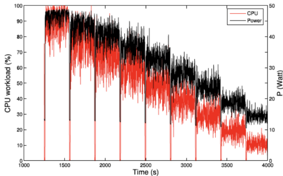
Fig. 5. The relationship between the CPU utilization and the power consumption of a D2581 Siemens-Fujitsu server running the SPEC Power (2008) benchmark [11].
