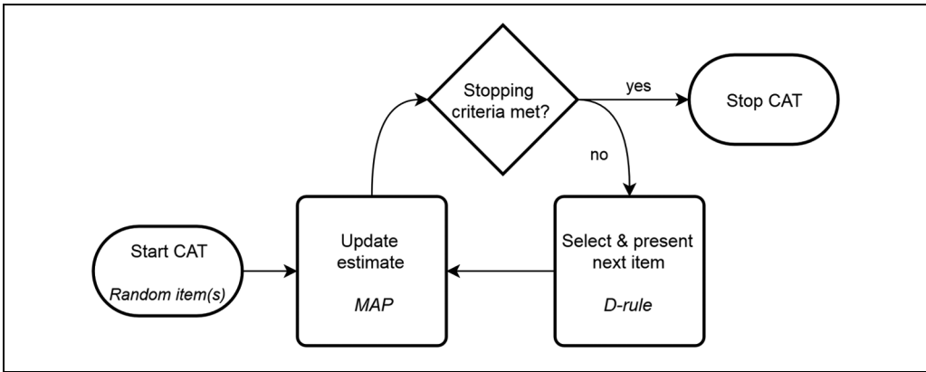
Figure 1. CAT flowchart.
