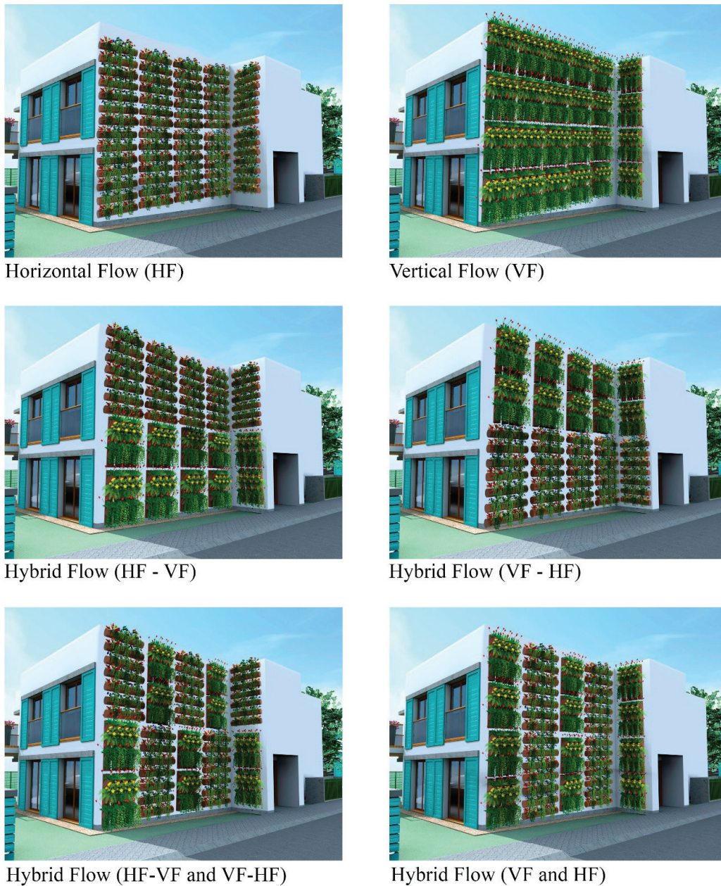
Fig. 3. The WETWALL design concept – possible treatment configurations.
