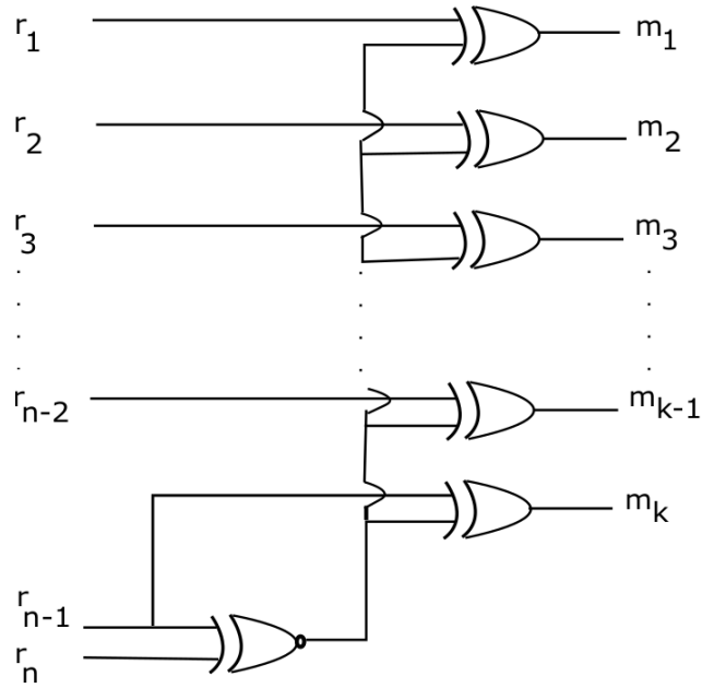
Figure 4.3: Decoder structure of the proposed UMLBI/CMLBI algorithm.
