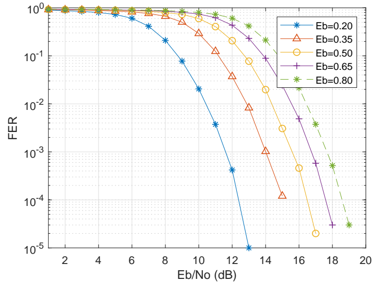
Figure 4.7: FER performance of proposed UMLBI/CMLBI code with varying SNR for k=100 .
