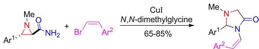
Scheme 3. Ring expansion reaction of aziridines
