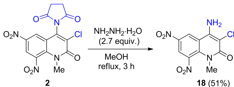
Scheme 10. Hydrazinolysis of imidated product 2
