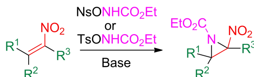
Scheme 8. Aziridination of nitroalkenes with \text{NsONHCO}_2\text{Et} or \text{TsONHCO}_2\text{Et}
