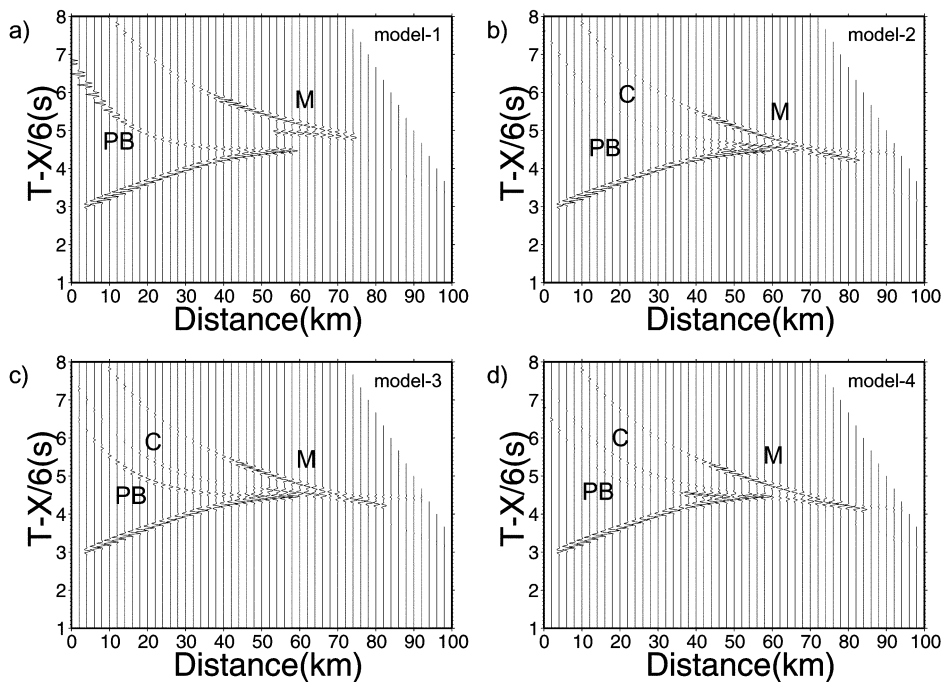
Fig. 4. Ray theoretical synthetic seismograms calculated from four different seismic structure models. Waveforms for model-1 to model-4 are shown in a) to d), respectively. Indexes denoting later arrivals are the same as in the observed record sections in Fig. 2. Direct water waves, reflections from the acoustic basement, and multiple reflections are not calculated.
