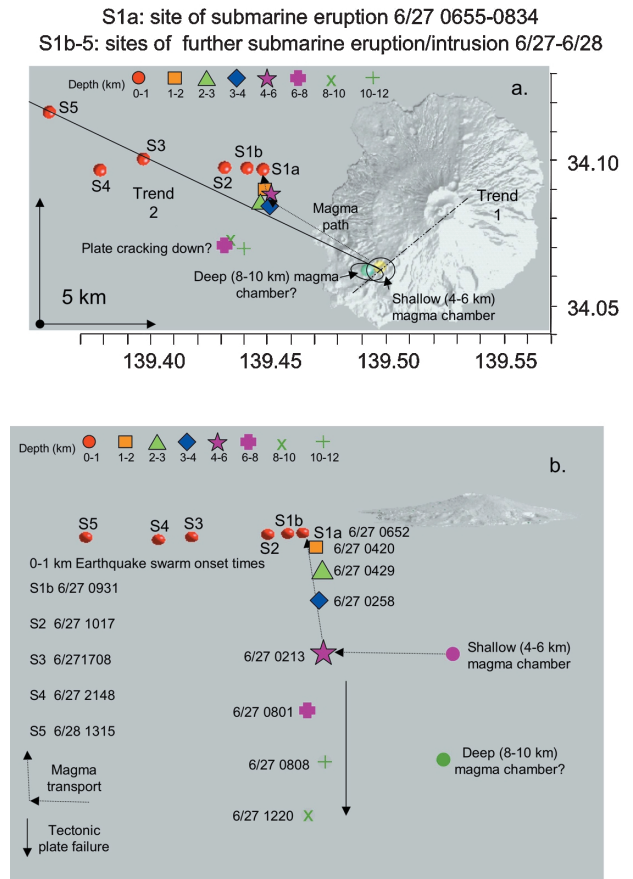
Fig. 3. Sites of eruption and/or shallow intrusion along trend 2 that are inferred to be fed from a shallow magma reservoir beneath the SW flank of Miyakejima. Magma chamber locations are inferred from seismicity associated with explosive eruptions at Miyakejima’s summit in August 2000. See text for further explanation.
