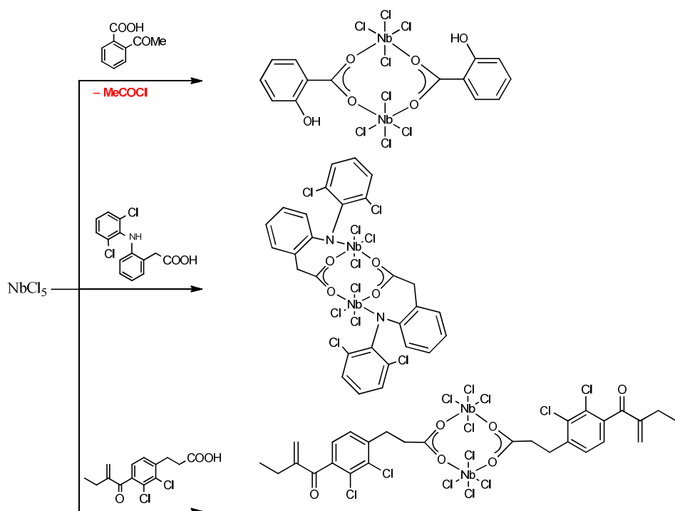
Scheme 5. Overview of the reactivity of \text{NbCl}_5 with bioactive carboxylic acids.
