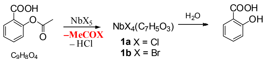
Scheme 1. Reaction of \text{NbX}_5 ( X = \text{Cl}, \text{Br} ) with acetylsalicylic acid.
