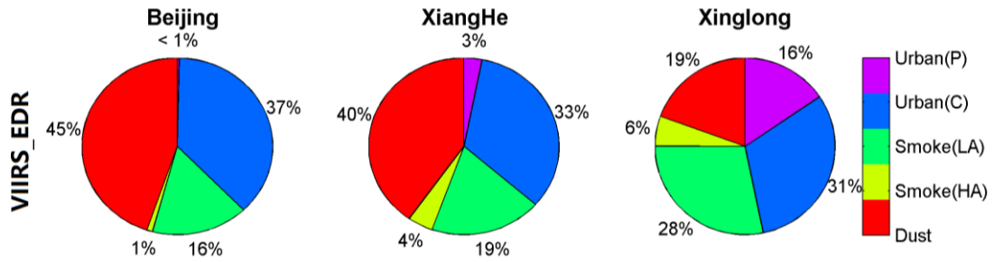
Figure 2. The frequencies of the aerosol model types used in the VIIRS_EDR at Beijing, XiangHe and Xinglong. Urban(P) is the polluted urban aerosol model, Urban(C) is the clean urban aerosol model, Smoke(LA) is the low absorption smoke aerosol model, Smoke(HA) is the high absorption smoke aerosol model, and the last aerosol model is for Dust.
