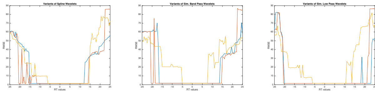
Figure 4: Comparison of algorithms for WA lidar-to-optical experiments (from left to right: splines, Simoncelli band-pass, Simoncelli low-pass); blue is wavelets, yellow is hybrid shearlets+wavelets with decomposition, and red is shearlets+wavelets without decomposition.
