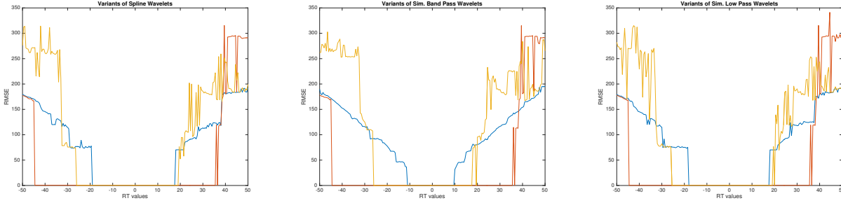
Figure 2: Comparison of algorithms for Mossy Rock synthetically warped experiments (from left to right: splines, Simoncelli band-pass, Simoncelli low-pass ); blue is wavelets, yellow is hybrid shearlets+wavelets with decomposition, and red is shearlets+wavelets without decomposition.
