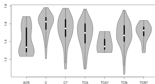
Figure 3: Violon plot and associated boxplots of fractal dimension for each group of IDPs in catalog 15.
