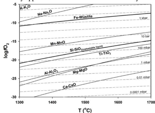
Figure 1. Plot of oxygen fugacity ( f_{\text{O}_2} ) vs. temperature ( T ) over the range of estimated liquidus temperatures of lavas on Mercury. Dashed lines represent the f_{\text{O}_2} of the GCO buffer at specified partial pressures of CO. The solid black lines represent the oxygen fugacities of various metal-metal oxide reactions at 1 bar. The wüstite in the iron-wüstite reaction represents \text{Fe}_{0.947}\text{O} , and the \text{SiO}_2 in the Si- \text{SiO}_2 reaction represents a metastable \text{SiO}_2 melt. Thermodynamic data for all of the calculations obtained from JANAF tables [9].
