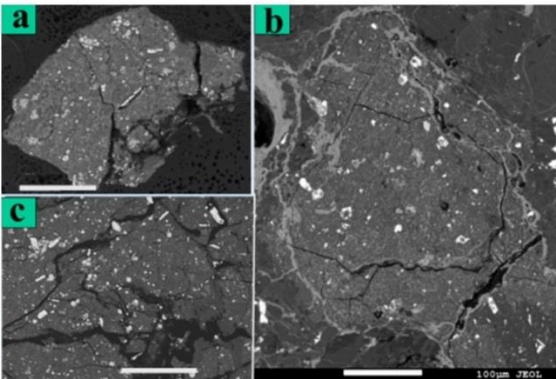
Figure 1. BSE images of three carbonaceous chondrite clasts in H chondrites. At this scale all that can be discerned is phyllosilicate (dark grey) and magnetite and pyrrhotite (white). (a) Clast in Tsukuba, (b) Clast in
