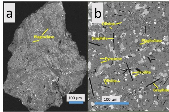
Figure 2. Melt clasts from two ordinary chondrites. (a) Melt clast in Zag. (b) Graphite- (black) bearing melt clast in NWA 6169. Scale bars are 100 μm.
