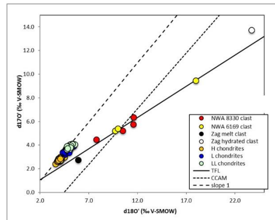
Figure 3. Oxygen 3 isotope plot of hydrated (CC) clast in Zag and melted clasts in H and L chondrites. Positions of ordinary chondrites are shown for comparison.
