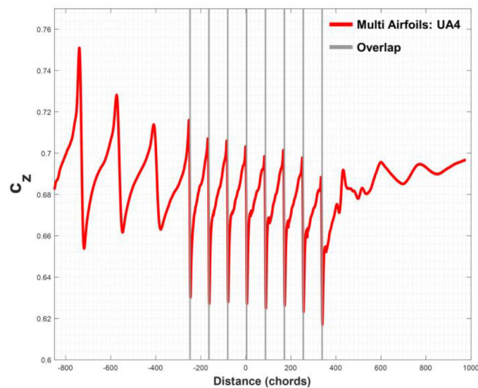
Figure 10. Multi airfoils crossing simulation of UA4 crossing lower airfoils 1-8 for c_z versus distance to overlap (Modern: M = 0.627 ( V_{tip} = 700 ft/s), \alpha = 5^\circ , S/c = 4 ( S = 2 ft, c = 0.5 ft), and D/c = 83.8 ( D = 41.9 ft)).
