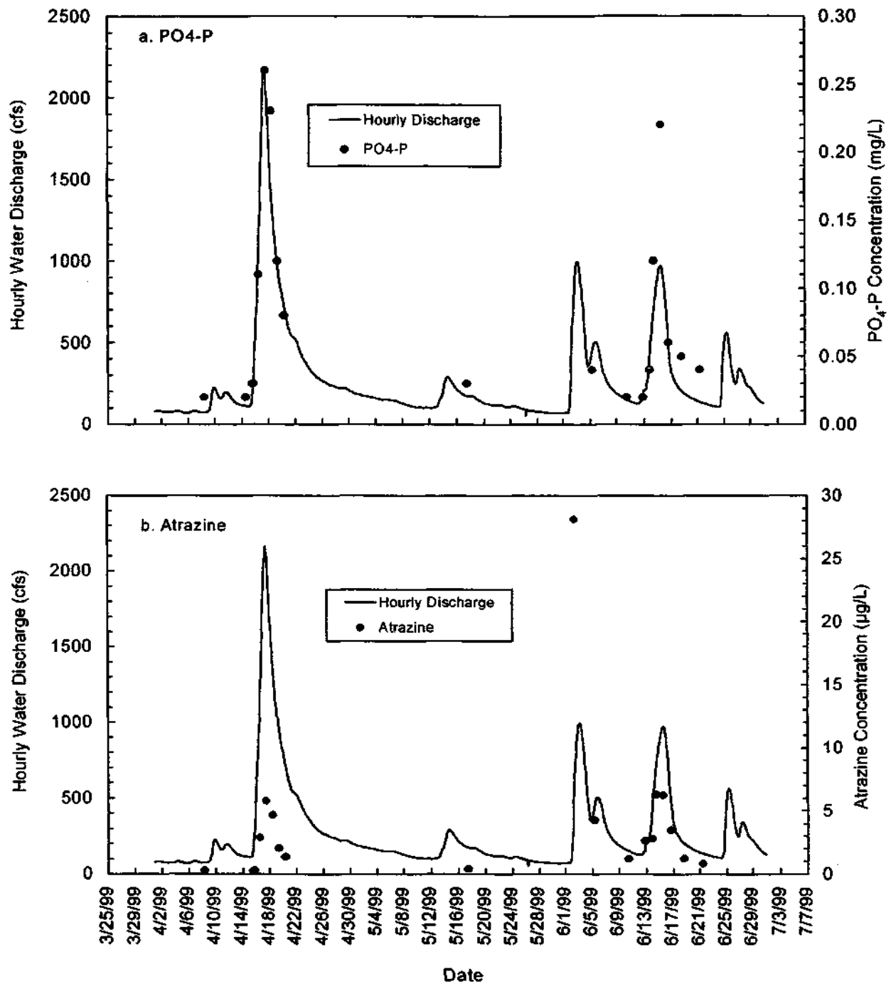
Figure 15. Observed data at Fisher monitored during 1999 storms: (a) hydrograph and concentrations of phosphate-phosphorous and (b) hydrograph and concentrations of atrazine
