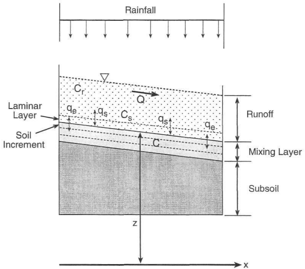
Figure 5. Schematic of chemical transport through rainfall-runoff and soil-chemical interactions (after Ashraf and Borah, 1992)
