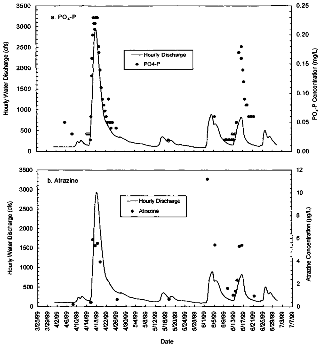
Figure 17. Observed data at Mahomet monitored during 1999 storms: (a) hydrograph and concentrations of phosphate-phosphorous and (b) hydrograph and concentrations of atrazine
