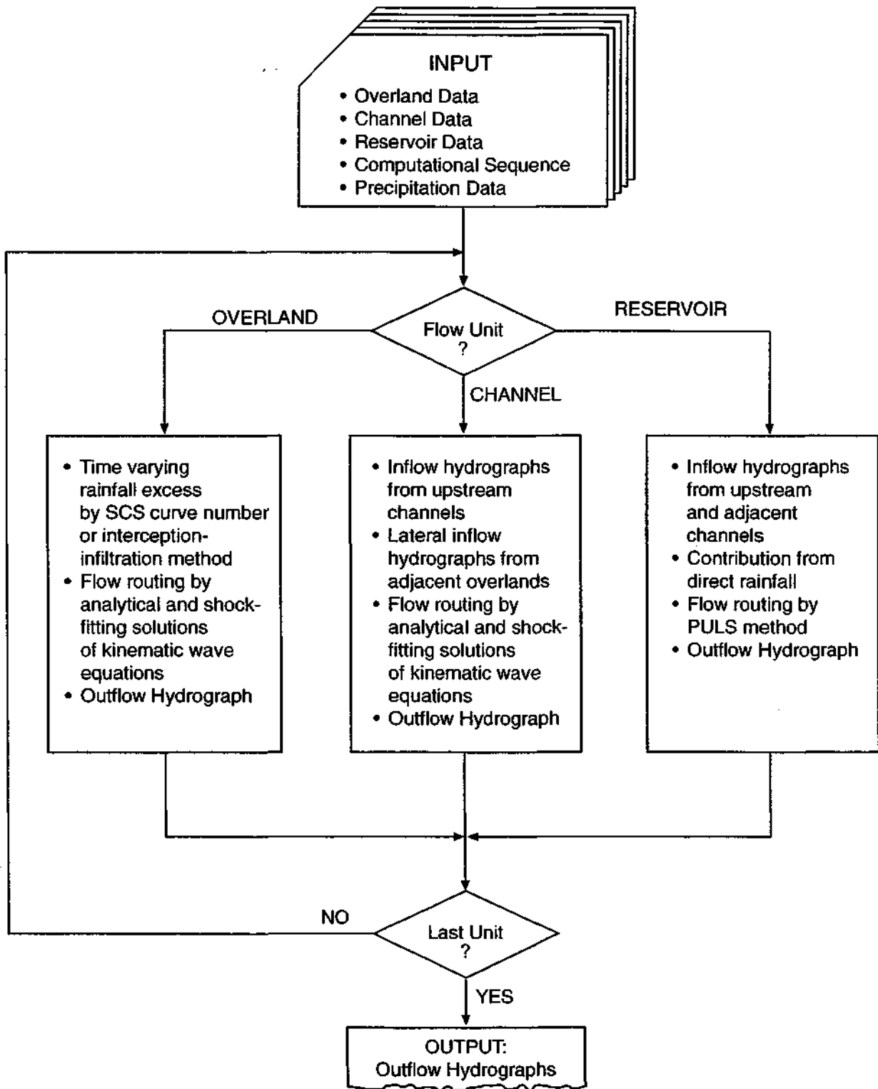
Figure 2. Flow diagram of hydrologic model
