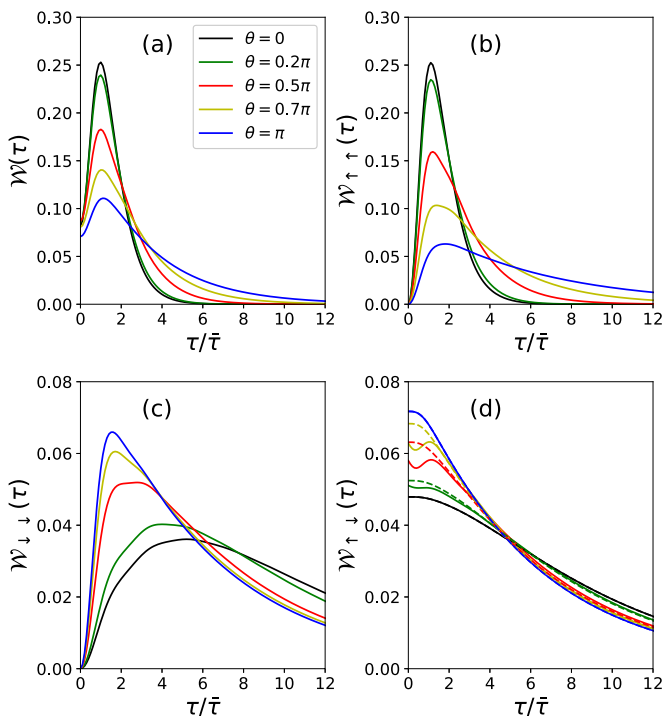
FIG. 3. (a) Two-channel WTD \mathcal{W}(\tau) , (b) spin-up WTD \mathcal{W}_{\uparrow\uparrow}(\tau) , (c) spin-down WTD \mathcal{W}_{\downarrow\downarrow}(\tau) , and (d) cross-channel WTD \mathcal{W}_{\uparrow\downarrow}(\tau) are plotted by varying noncollinear angle \theta with spin polarization p = 0.8 . The corresponding FPTD for spin-down \mathcal{F}_{\downarrow}(\tau) is plotted with a dashed line in (d). The waiting time is in units of time, \bar{\tau} = h/(eV) .
