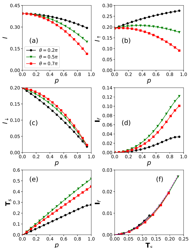
FIG. 7. (a) Charge current, (b) spin-up current I_{R\uparrow} , (c) spin-down current I_{R\downarrow} , (d) influence degree, and (e) \mathbf{T}_s vs spin polarization p with different noncollinear angles \theta . (f) Influence degree vs \mathbf{T}_s with the quadratic fitting \mathbf{I}_f = 0.51(\mathbf{T}_s)^2 shown as dashed lines.
