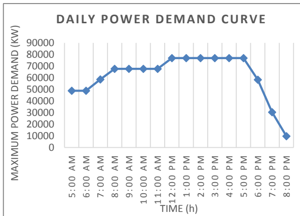
Figure 8: Daily power demand curve developed by using model 3
