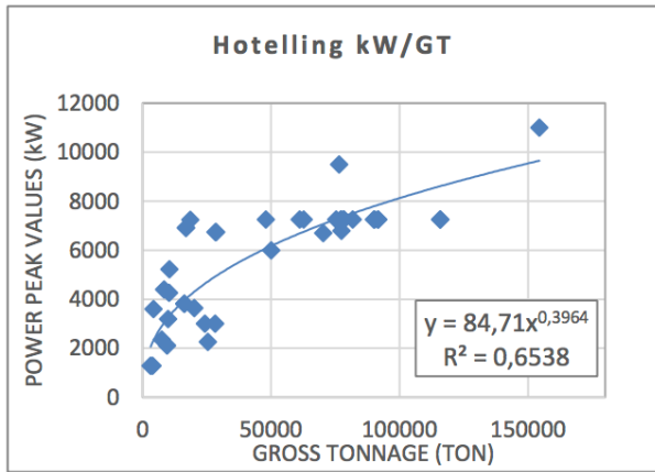
Figure 5: Model 3 - Hoteling/Gross tonnage ratio by potential regression. Obtained correlation factor of 0.808
