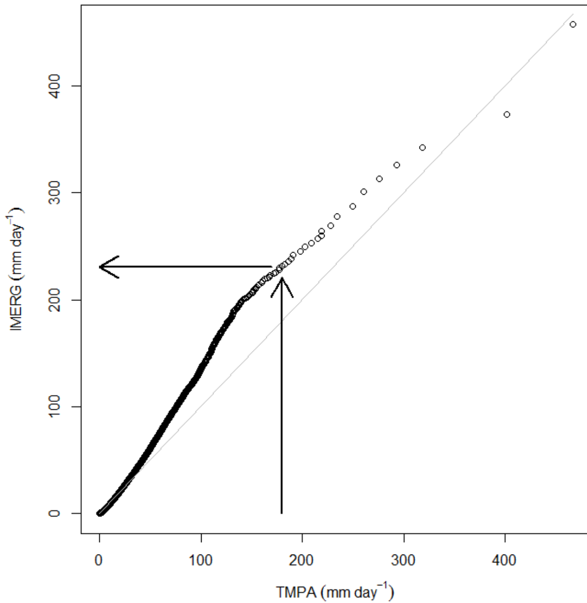
290 Figure 2: Quantile-quantile plot for the Central American land area for May 6, 2015-May 5, 291 2015. 100,000 quantiles (open circles) were calculated for the TMPA-RT and IMERG-L rainfall 292 estimates. In quantile mapping, a value from one product is used to look up the value of the
