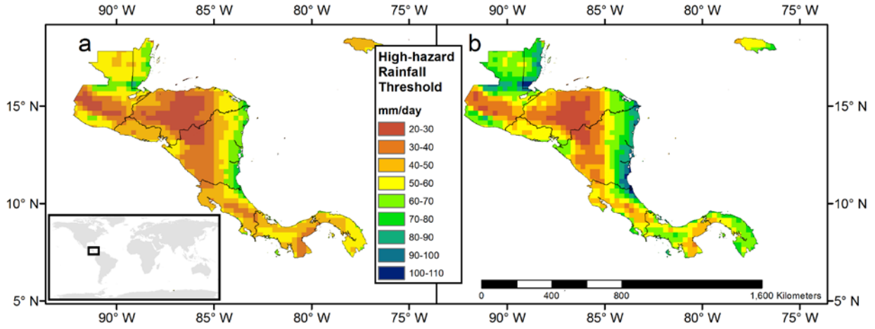
297 Figure 3: The LHASA high-hazard rainfall threshold was calculated from a) TMPA-RT data for the 298 period 2001-2014, b) the quantile-mapped IMERG-L equivalent thresholds.
