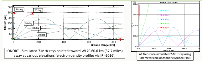
IONORT - Simulated 7-MHz rays pointed toward WL7C 60.6 km (37.7 miles) away at various elevations (electron density profiles via IRI-2016).
