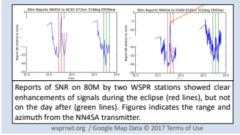
Reports of SNR on 80M by two WSPR stations showed clear enhancements of signals during the eclipse (red lines), but not on the day after (green lines). Figures indicate the range and azimuth from the NN4SA transmitter.
