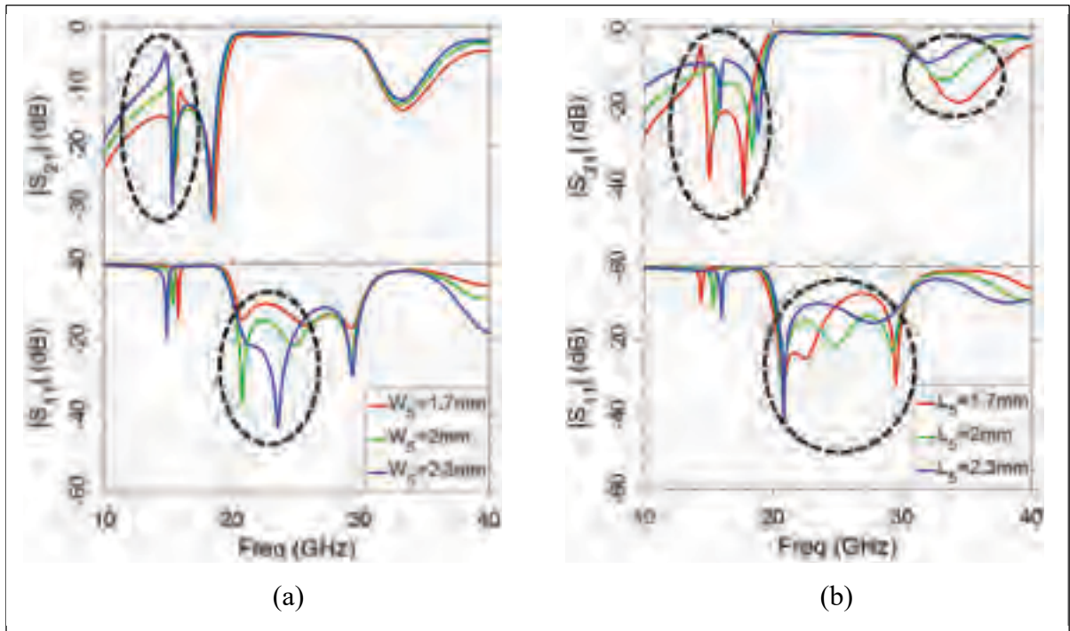
Figure 3.12 Effect of the common ground aperture dimensions: (a) variations of W_5 while L_5=2 mm b) variations of L_5 while W_5=2 mm
