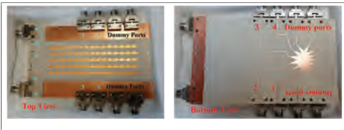
Figure 5.16 Top (left) and bottom (right) view of the fabricated structure
