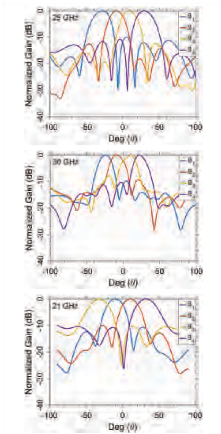
Figure 5.13 x-z Plane Normalized gain for beam ports 1 to 4 excitation
