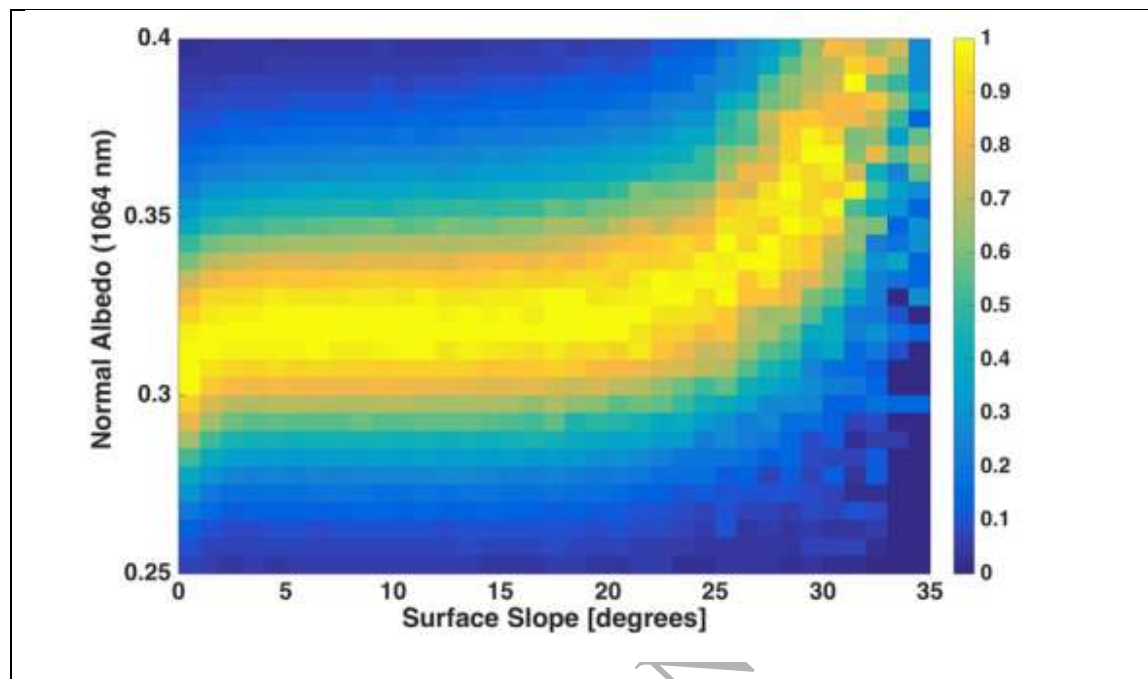
Figure 3. Two-dimensional histogram that displays mode-normalized LOLA reflectance distribution as a function of surface slope for the North and South pole. Reflectance bin width=0.005 and slope bin width=1 degree . The strong influence of surface slope is a potential source of temperature-independent bias on the reflectance-temperature relationships observed in the polar regions. [1 column]
