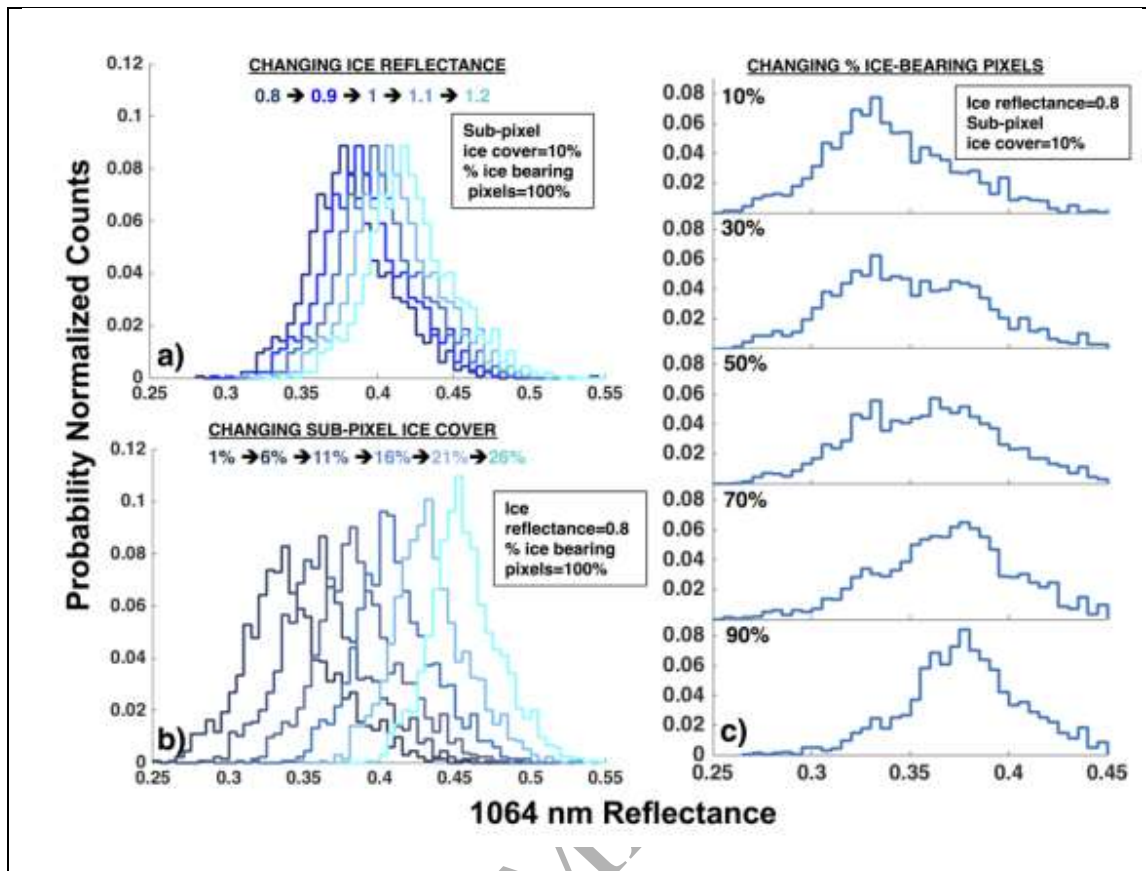
Figure 9. Results showing the effect of varying our three ice model input parameters: ‘ice reflectance’ (a), ‘sub-pixel ice cover’ (b), and ‘percent ice bearing pixels’ (ice-heterogeneity)(c). This model applies ice-brightened material to an ice free distribution via linear mixing. The ice-free starting distribution was we chose the reflectance distribution of low slope (slope <10^\circ ) South-polar PSRs (average incident flux=0%), with maximum temperatures high enough ( >125\text{K} ) to preclude the preservation of surface ice. Reflectance bin width of all histograms equals 0.005. [1.5 column]
