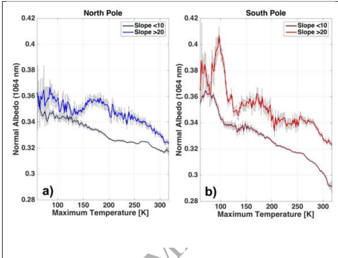
Figure 4. Average 1064 nm reflectance as a function of maximum temperature for low slope (slope < 10^\circ ) and high slope (slope > 20^\circ ) areas for the North (a) and South (b) polar regions. Maximum Temperature bin width=2K. Reflectance average plotted with 2\sigma errors (standard error of the mean). [1.5 column]
