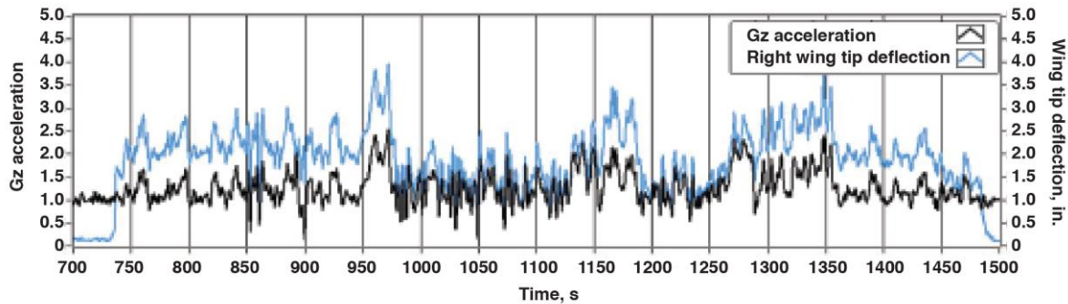
Figure 19. Filtered (nine-point moving average), vertical acceleration in g's (black) and right wing-tip deflection (blue).
