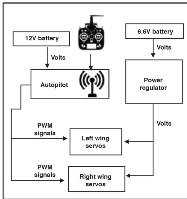
Figure 5. System block diagram for the wing control surfaces of the baseline aircraft.
