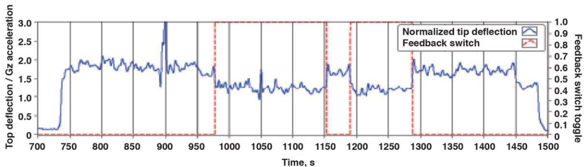
Figure 20. Tip deflection normalized by vertical acceleration (blue) and control algorithm toggle switch signal showing when the feedback was turned on and off (red).
