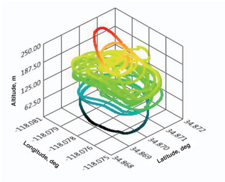
Figure 15. Flight profile; the color spectrum has been mapped as a function of altitude.
