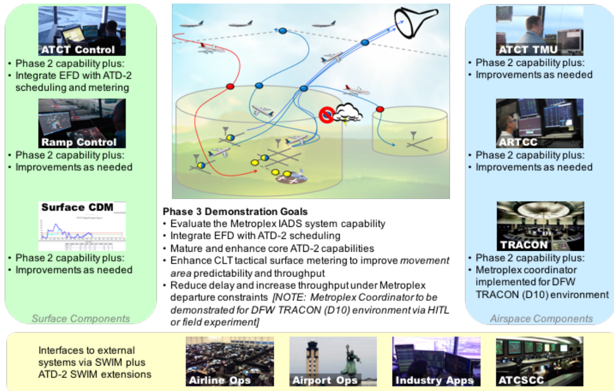
Figure 36 - This full operational overview of the IADS system highlights both the participants at various facilities and the system improvements for the Phase 3 Metroplex IADS Demonstration.
