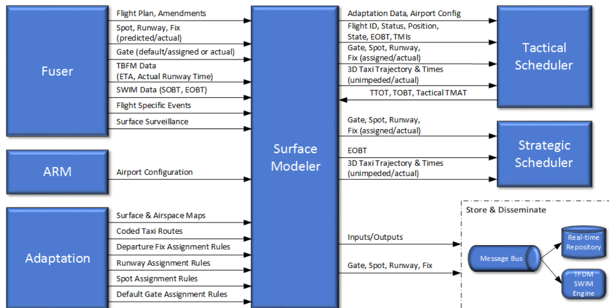
Figure 16 – The ATD-2 Surface Modeler component consumes/produces a variety of data.
