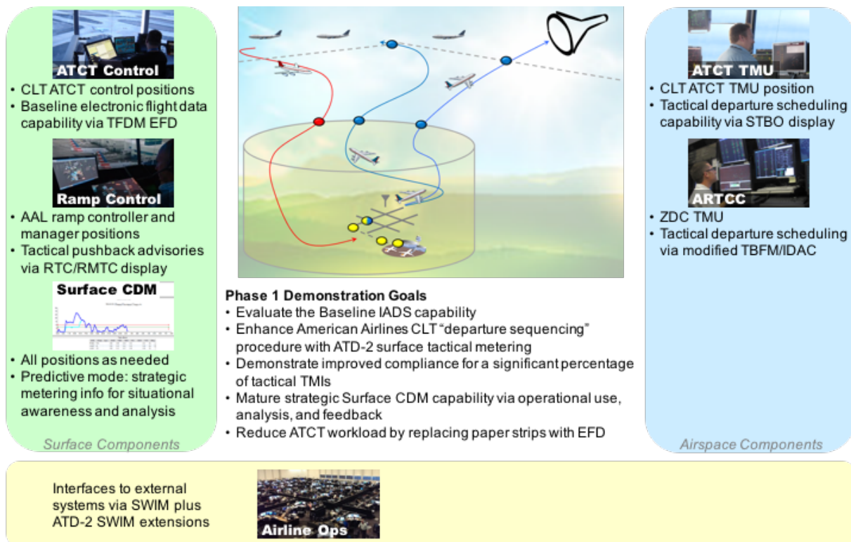
Figure 34 - This operational overview of the IADS system highlights both the participants at various facilities and the system improvements for the Phase 1 Baseline IADS Demonstration.
