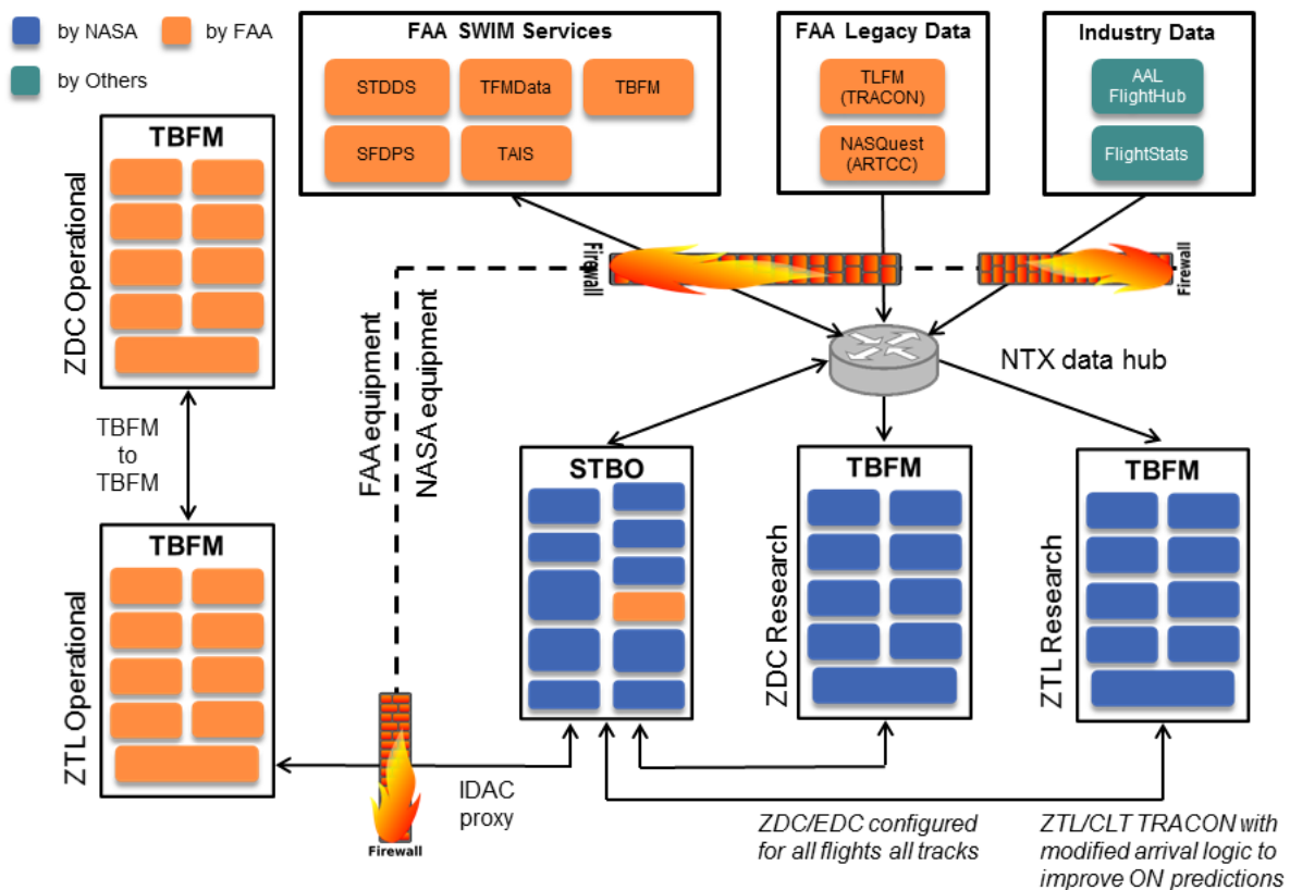
Figure 28 - The relationship among the TBFM and STBO systems is shown in the NASA proposed solution.
