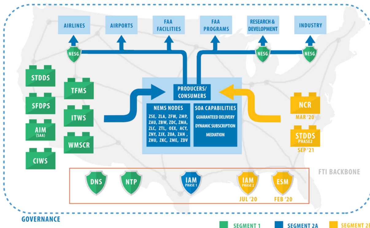
Figure 9 - System Wide Information Management (SWIM) is being implemented in segments [as briefed to NASA in July 2016].
