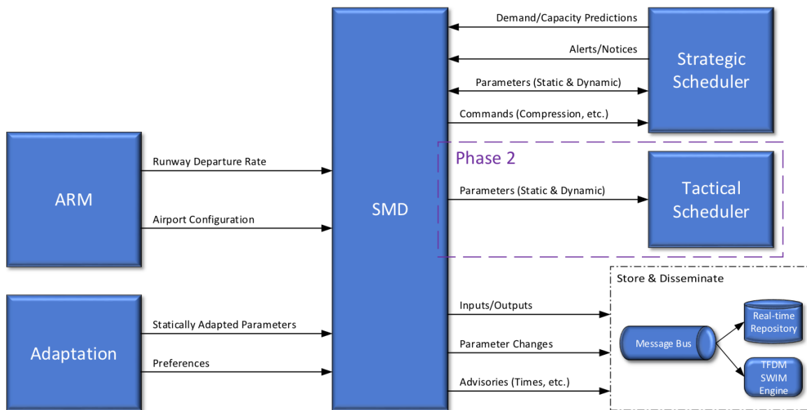
Figure 20 - The SMD user interface component consumes/produces a variety of data.
