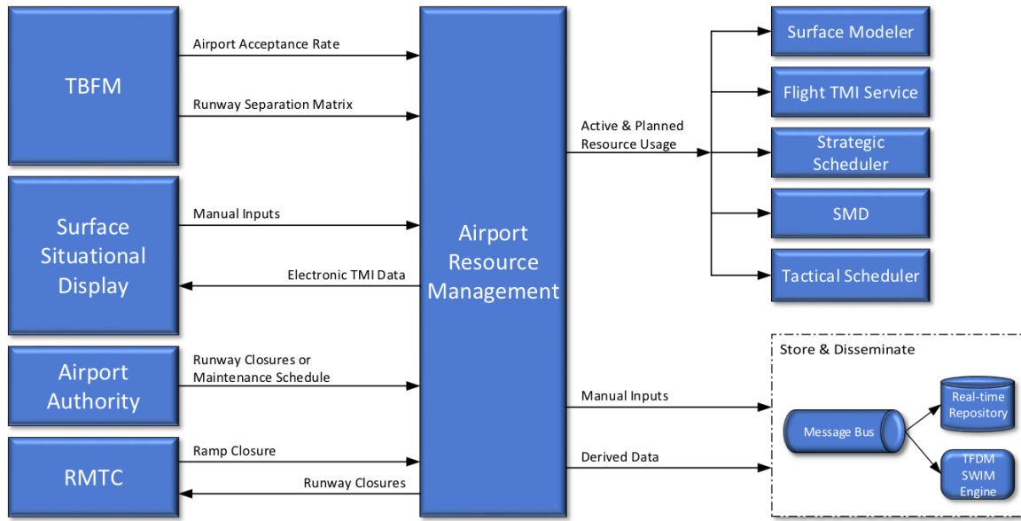
Figure 24 - The Airport Resource Management component consumes/produces a variety of data.
