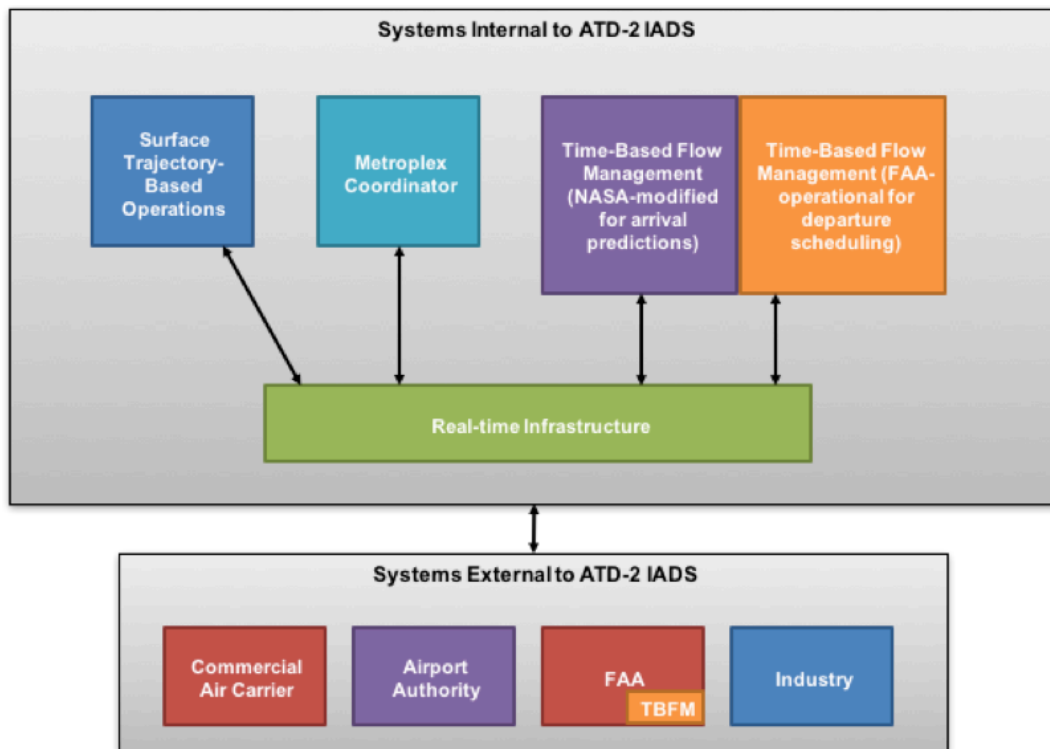
Figure 13 - This simplified view of the ATD-2 IADS architecture shows only the major components.
