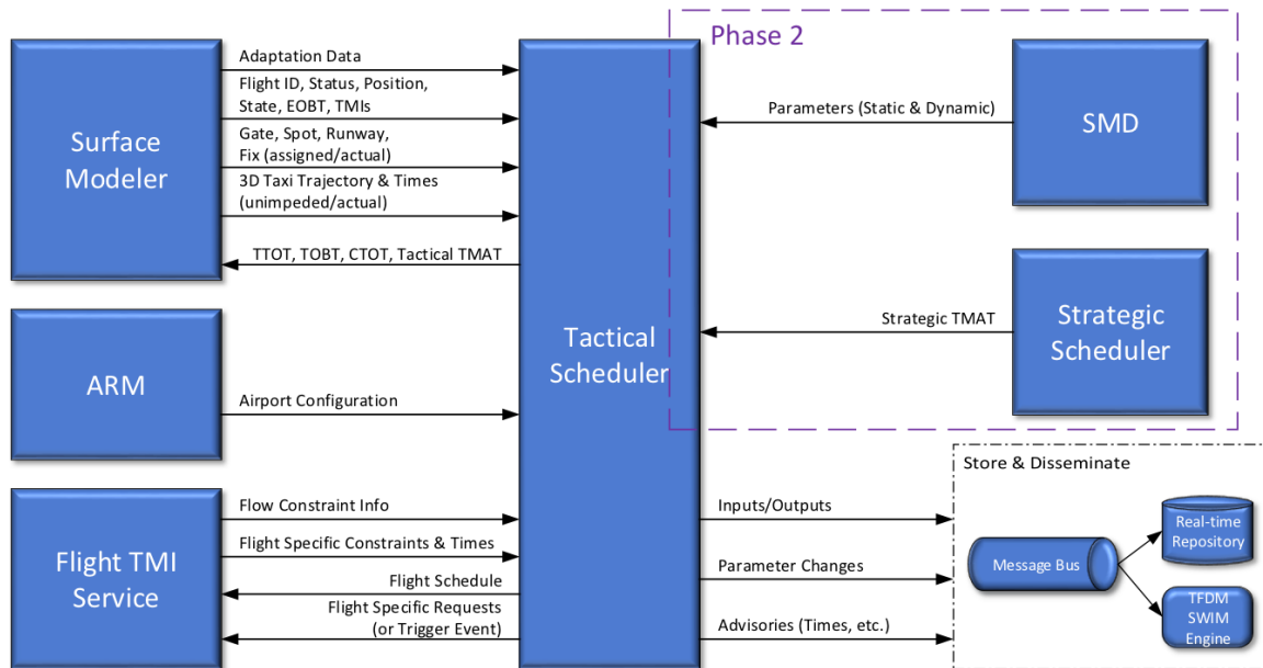
Figure 18 – The Tactical Scheduler component consumes/produces a variety of data.
