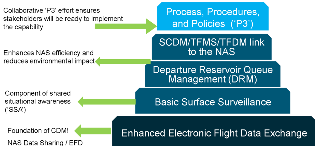
Figure 8 - The Surface CDM component of TFDM will implement a collaborative departure queue management solution.
