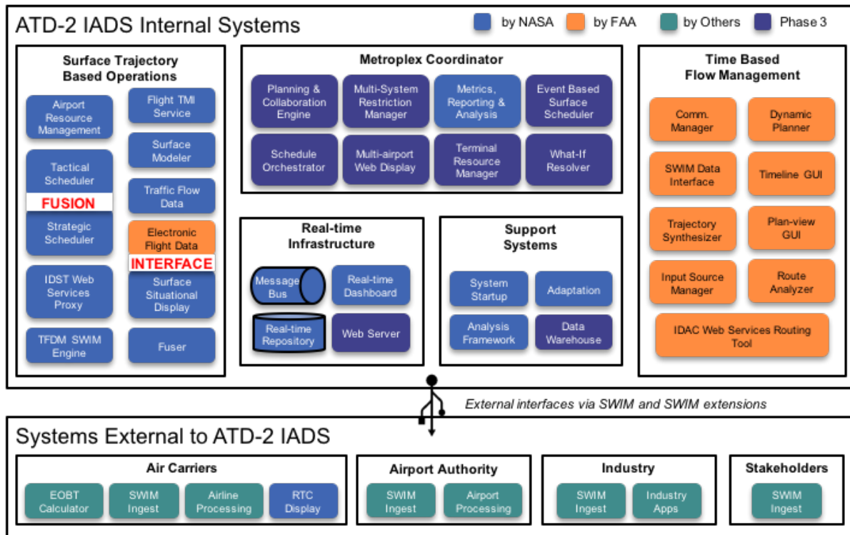
Figure 14 - The logical architecture for the IADS field demonstration system is shown to the next level of detail.
