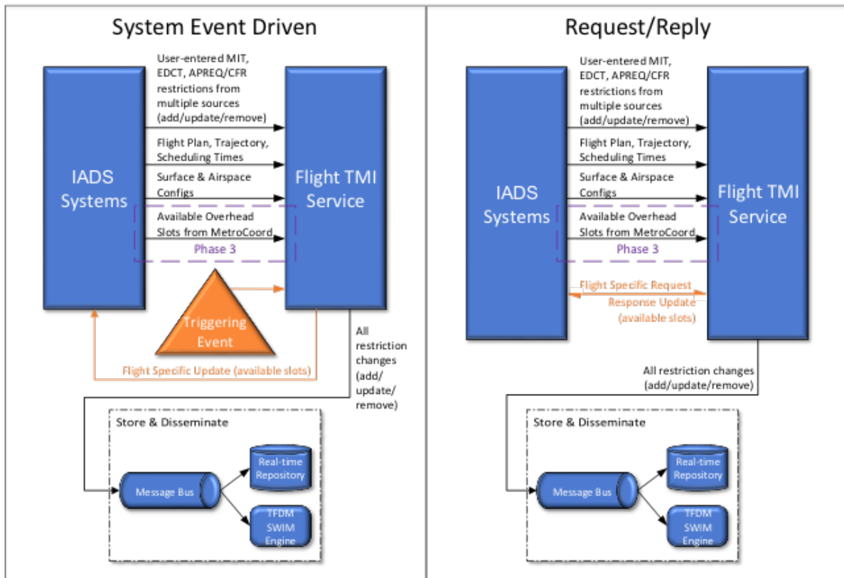
Figure 26 - An Event Driven data flow is shown in the left panel and a Request/Reply data flow mechanism is shown in the right panel for the Flight TMI Service component.
