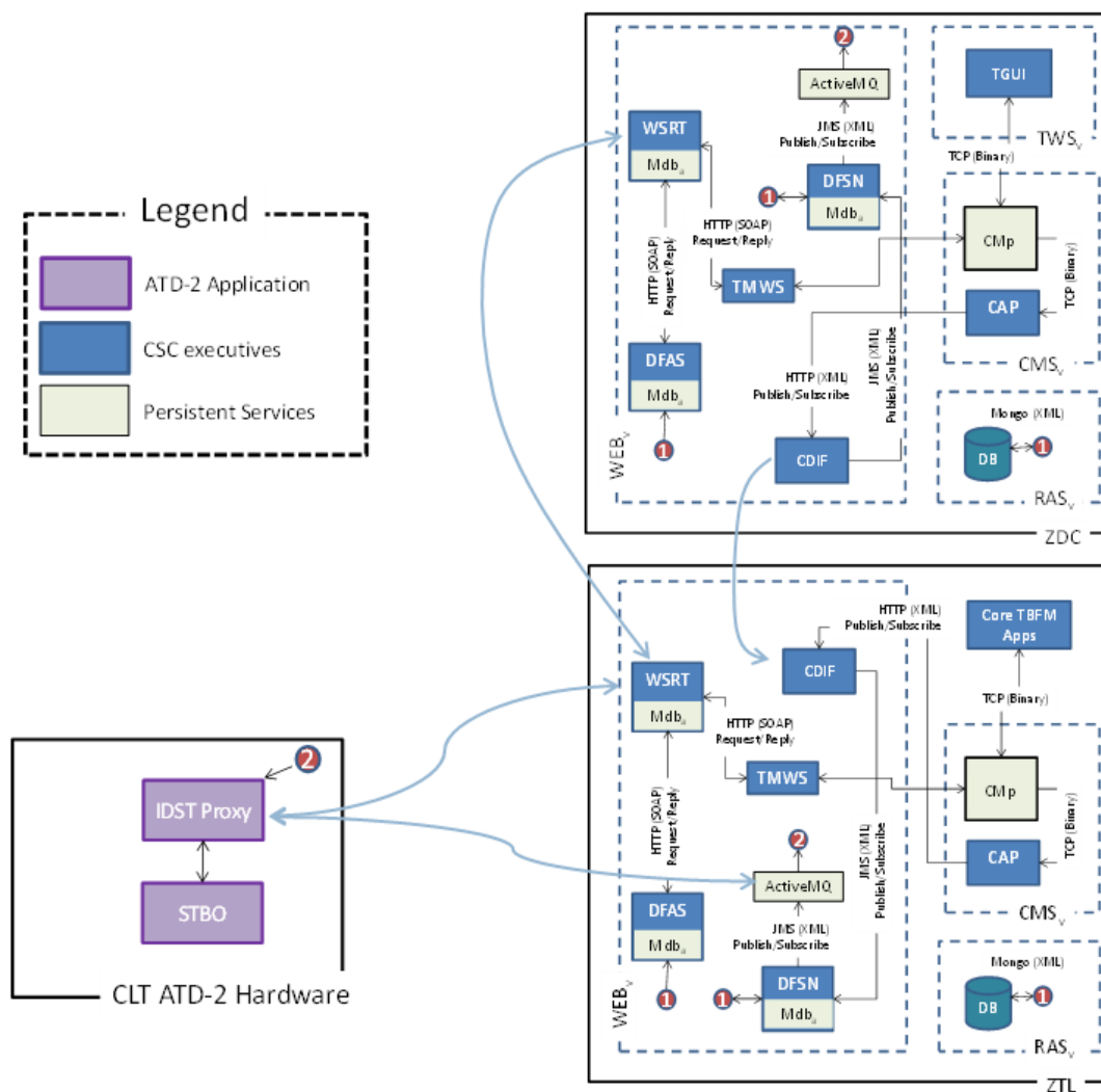
Figure 29 - Lockheed Martin proposes a solution leveraging TBFM-to-TBFM capability.
