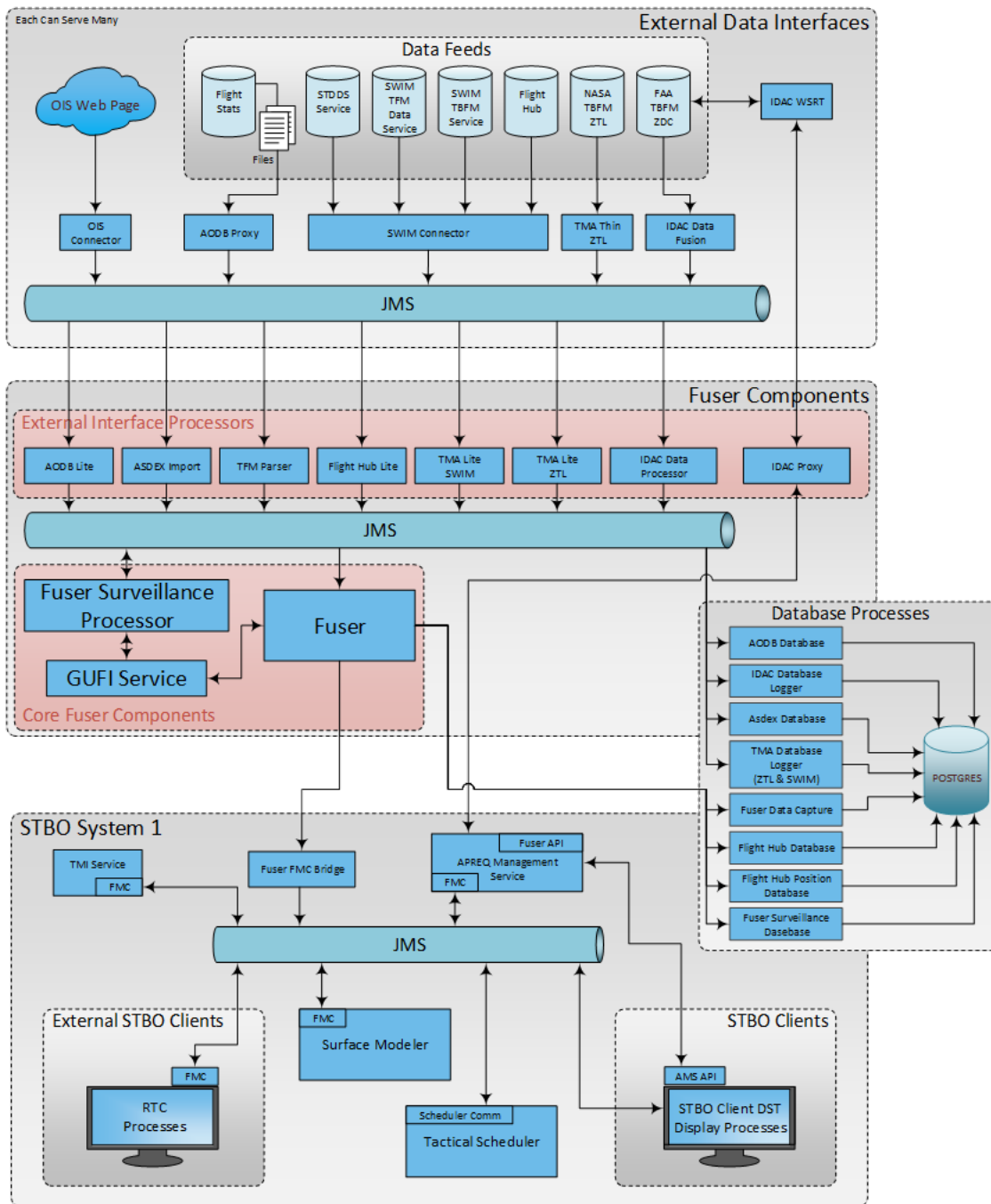
Figure 22 - The Fuser architecture overview shows the communication flow of the sub-components that comprise the Fuser system.
