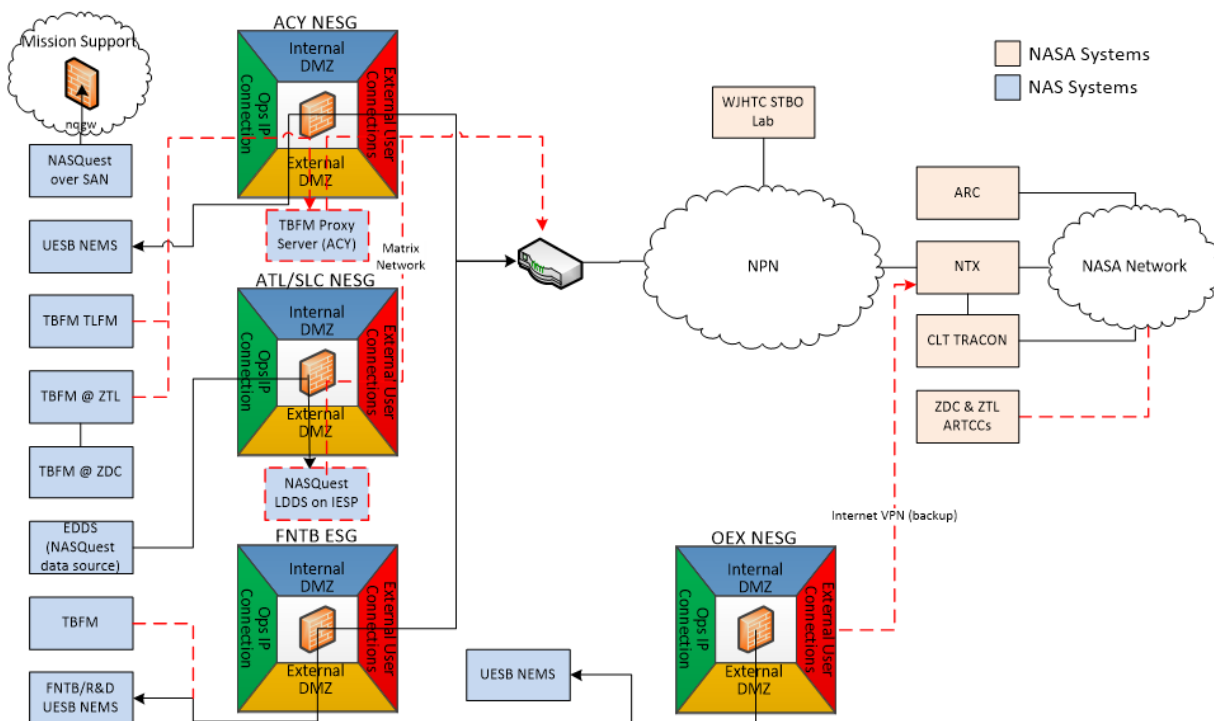
Figure 31 – This figure highlights the interfaces between FAA and NASA information systems for the ATD-2 field demonstration.
