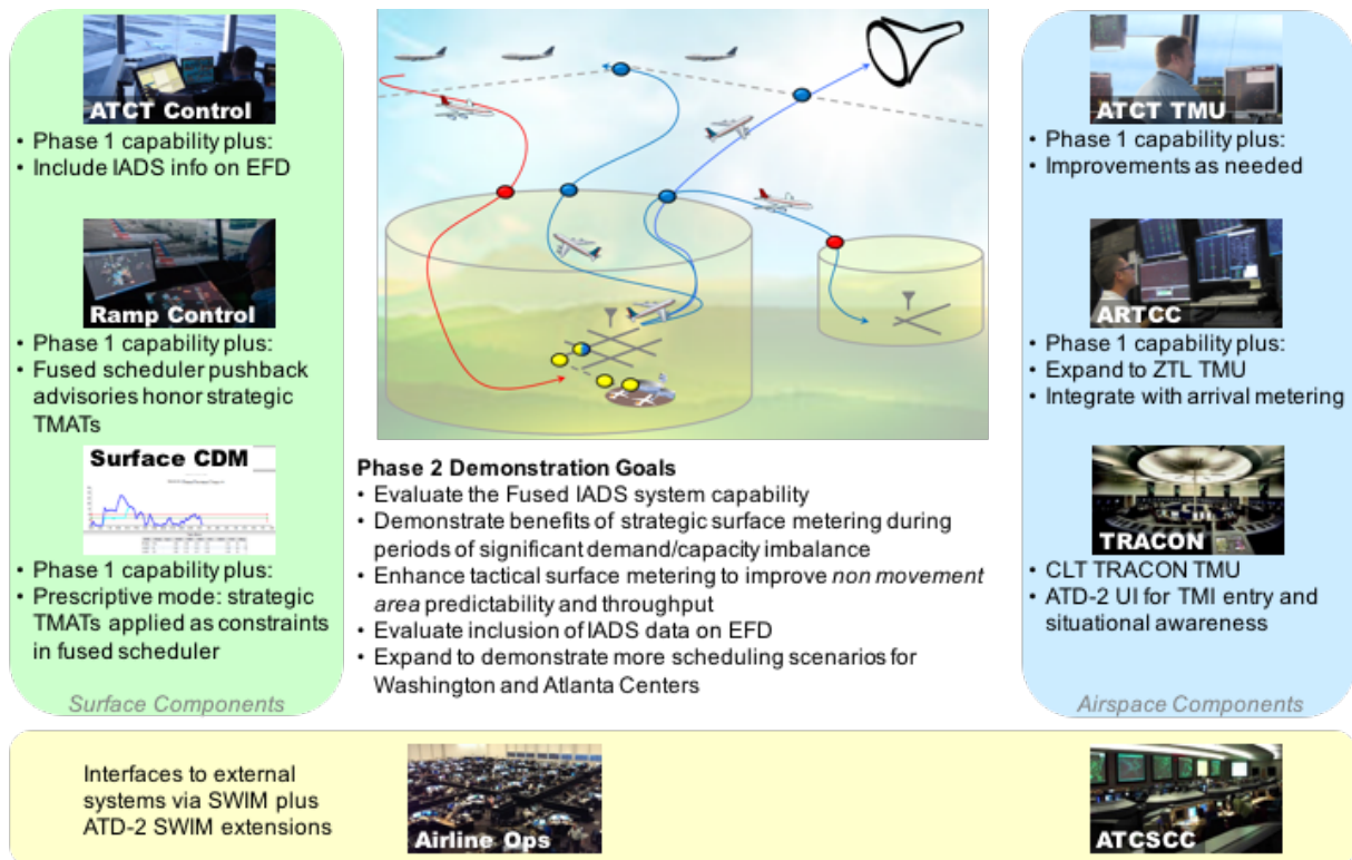
Figure 35 - This enhanced operational overview of the IADS system highlights both the participants at various facilities and the system improvements for the Phase 2 Fused IADS Demonstration.
