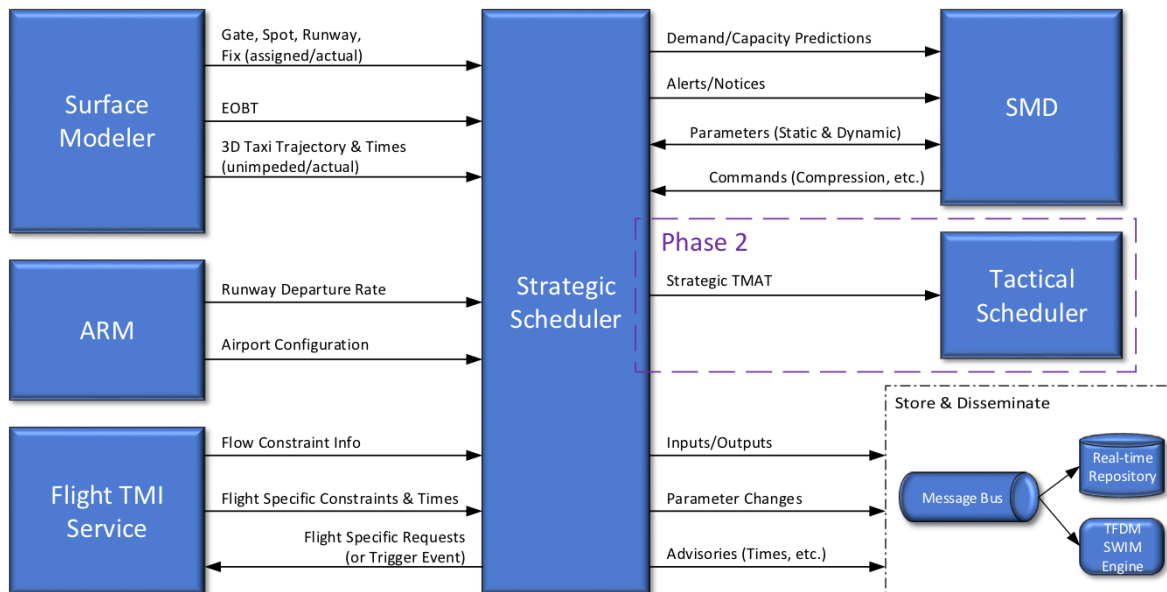
Figure 19 - The Strategic Scheduler component consumes/produces a variety of data.
