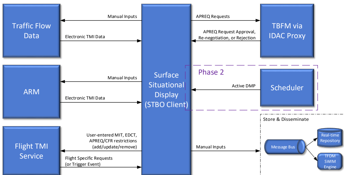
Figure 25 - The Surface Situational Display component consumes/produces a variety of data.
