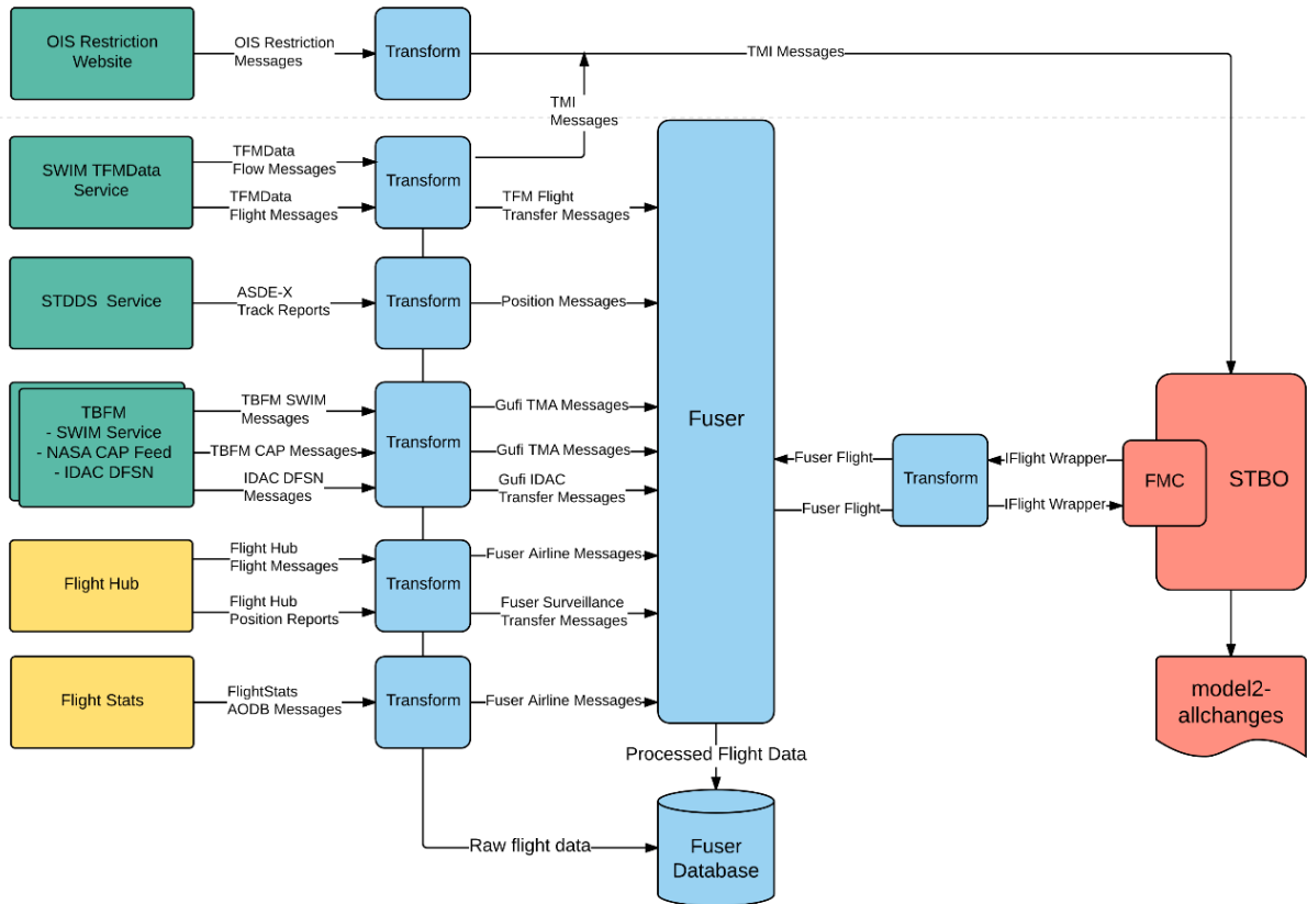
Figure 21 - This illustration shows the data flow to/from the Fuser.
