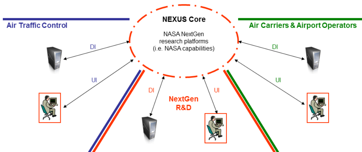
Figure 38 - NASA's information system security plan uses the NextGen Emulation system (NEXUS) abstraction to define system boundaries and two classes of system interfaces.
