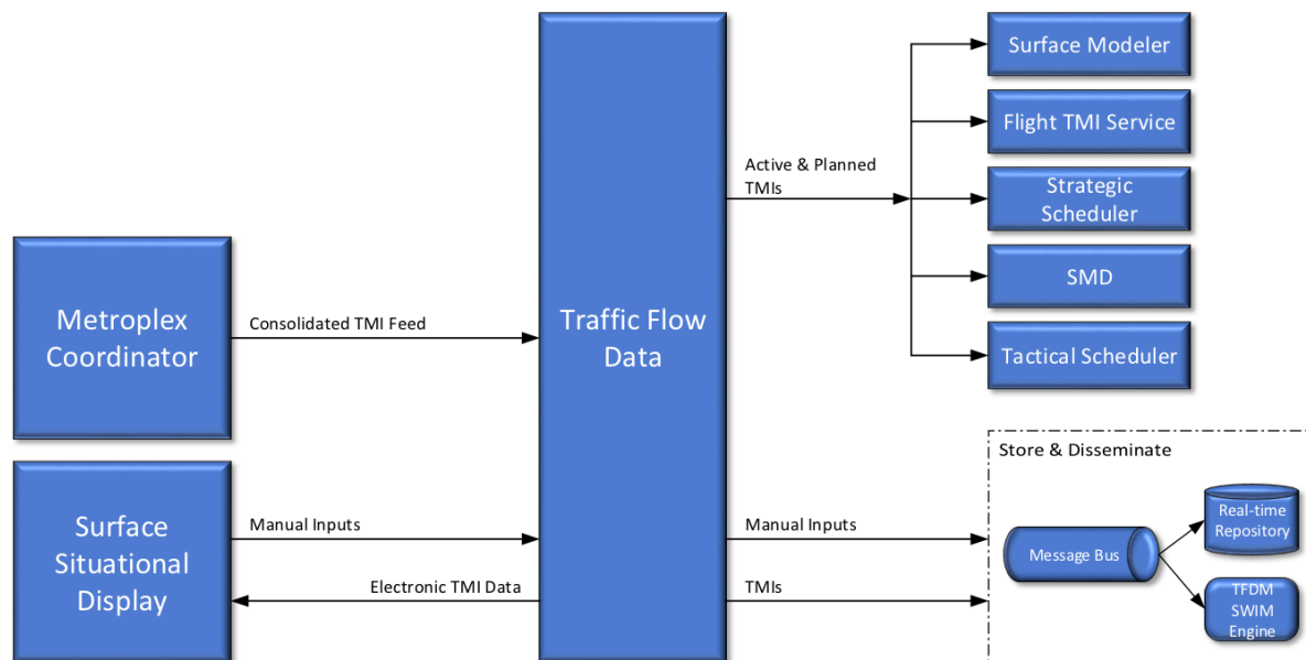
Figure 23 - The Traffic Flow Data Management component consumes/produces a variety of data.
