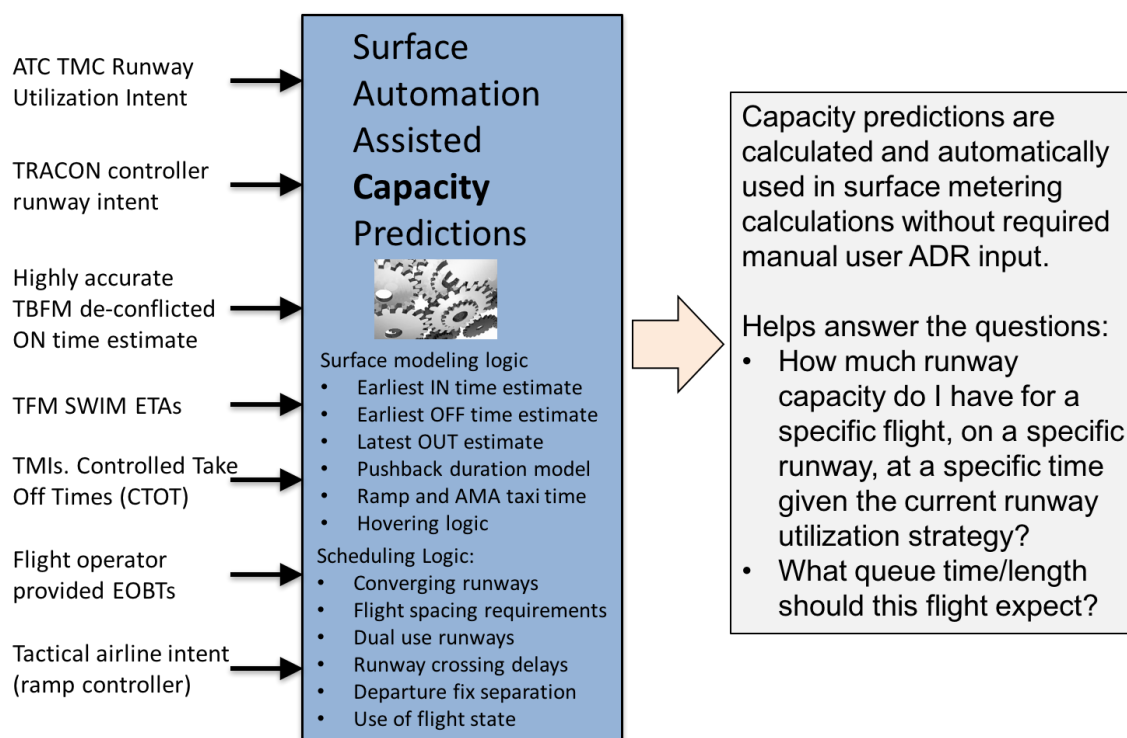
Figure 14 - The capacity prediction automatically updates the capacity of each runway, using various inputs, without relying on manual entries.
