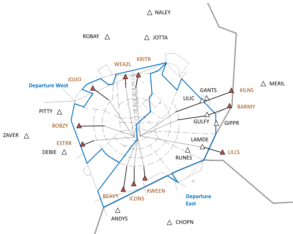
Figure 5 - CLT TRACON departure sectors and RNAV departure routes are shown.
