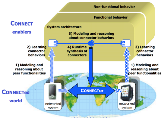
Fig. 2. The overall Connect process, including enablers
