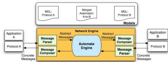
Fig. 3. The Starlink middleware technology
