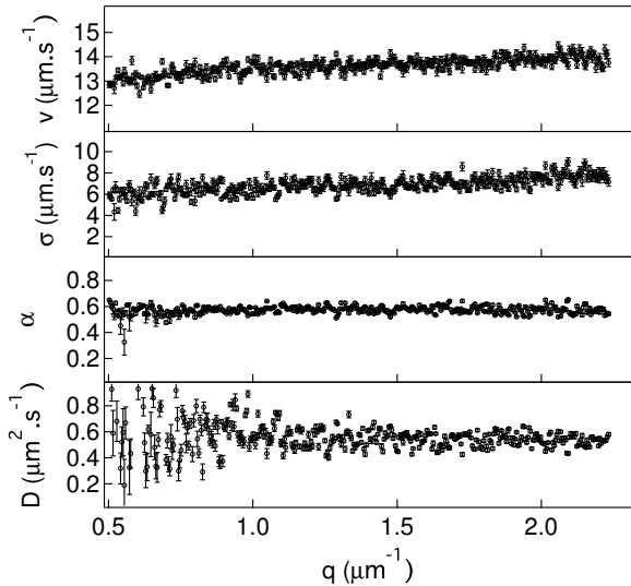
FIG. 3: Parameters extracted from fitting the DICF data for motile cells. From top to bottom: \bar{v} and \sigma of the Schulz distribution, motile fraction \alpha and diffusivity D .
