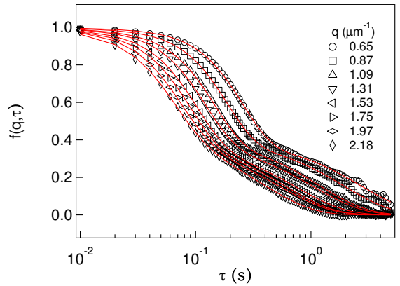
FIG. 2: Symbols: reconstructed ISFs for motile E. coli at 8 values of q spanning the whole available range (see key). Lines: calculated ISFs, Eqs. (8)-(11), using fitted parameters.
