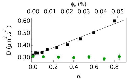
FIG. 4: ■: D as a function of \alpha (lower axis) and the volume fraction of swimmers, \phi_\alpha (upper axis). The black line is a linear fit. ●: D(\alpha) from simulations.
