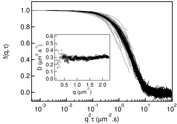
FIG. 1: Reconstructed ISFs of non-motile bacteria plotted against q^2\tau . Solid (black) curves for over 200 values of q in the range 0.5\mu\text{m}^{-1} \lesssim q \lesssim 2.2\mu\text{m}^{-1} collapse, but curves from lower q (grey) do not collapse. Inset: fitted diffusivity D(q) (black and grey with the same meaning).
