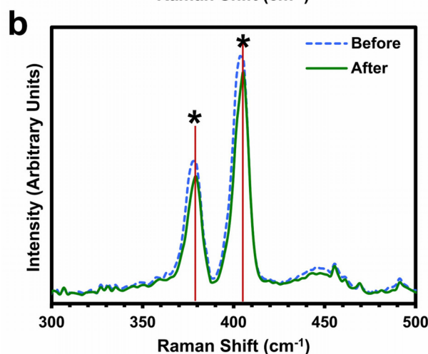
Fig. 8 Raman spectra acquired before and after Li + intercalation of two different MoS 2 flakes: (a) thickness ~10 nm and (b) thickness >20 nm. [*] represent the MoS 2 peak locations corresponding to the as deposited thin films.
