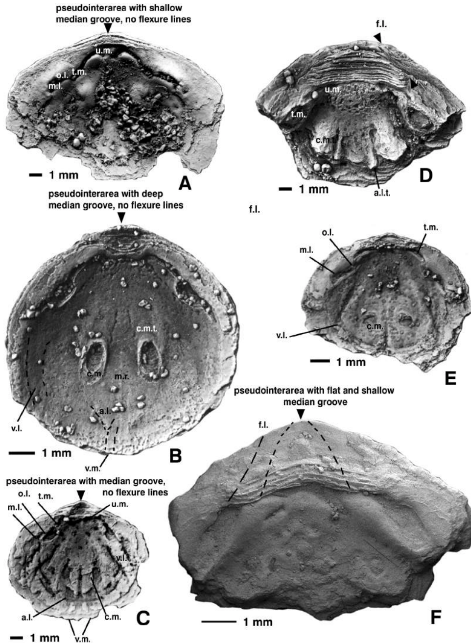
Figure 4: Main features of dorsal valve interior of Obolus and Ungula . A , Obolus transversus (PANDER, 1830), CNIGR 22/12348; Middle Cambrian, Sablinka Formation, Rebrovo Member, Sample L-41/3 (POPOV et alii , 1989, fig. 2), right-hand side of Volkhov River in southern outskirts of the village of Gorchakovshchina, St Petersburg District; note that mature specimen has low dorsal pseudointerarea occupied mainly weakly defined pedicle groove and lacks flexure lines, with paired umbonal muscle scars (u. m.) divided by short median ridge and posterolateral muscle fields slightly raised above the valve floor with attachment scars of transmedian (t.m.), oblique lateral (o.l.) and middle lateral (m.l.) muscles. B , Obolus apollinis EICHWALD, 1829; IGT, B1706; Upper Cambrian, lower Tosna Formation, sample L1/3 (POPOV et alii , 1989, fig. 3), right-hand side of lava River in southern outskirts of the village of Gorodishche, St Petersburg District; note narrow dorsal pseudointerarea, mainly occupied by median groove, very weak median ridge (m.r.) in anterior half of the visceral area, central muscle scars (c.m.) on the end of distinct tracks (c.m.t.) slightly raised above valve floor, but not forming platforms, anterior lateral muscle scars (a.l.) near the margins of the visceral area, proximal ends of weakly impressed, subparallel vascula media (v.m.) and arcuate vascula lateralia (v.l.). C , Obolus ruchini KHAZANOVITICH et POPOV, 1984; CNIGR 13/12348; Middle Cambrian, Sablinka Formation, Gertovo Member, Sample L6/1 (POPOV et alii , 1989, fig. 3), right-hand side of Sarya River about 700 m downstream from the northern outskirts of the village of Voibokalo, St Petersburg District; note muscle scars and impressions of mantle canals. D-F , Ungula convexa PANDER, 1830, Upper Cambrian, Ladoga Formation; D , CNIGR 126/12348, sample L9/31b (POPOV et alii , 1989, fig. 4), Naziya River, left-hand side near the abandoned village of Novaya, St Petersburg District; mature specimen ( cf. fig. 4A-B) with high pseudointerarea bearing broad flattened median groove separated from flexure lines (f.l.) on propleareas, paired umbonal muscle scars and transmedian muscle scars on raised platforms; distinct, raised tracks of central (c.m.t.) and anterior lateral muscles (a.l.t.) in the median part of the shell represent a distinctive pattern markedly different from Obolus ; E , CNIGR 129/12348; sample L47/4 (POPOV et alii , 1989, fig. 5), Izhora River, left-hand side, about 800 m upstream of the locality B2; juvenile specimens with raised muscle tracks and platforms not yet formed, but with well impressed muscle scars and
