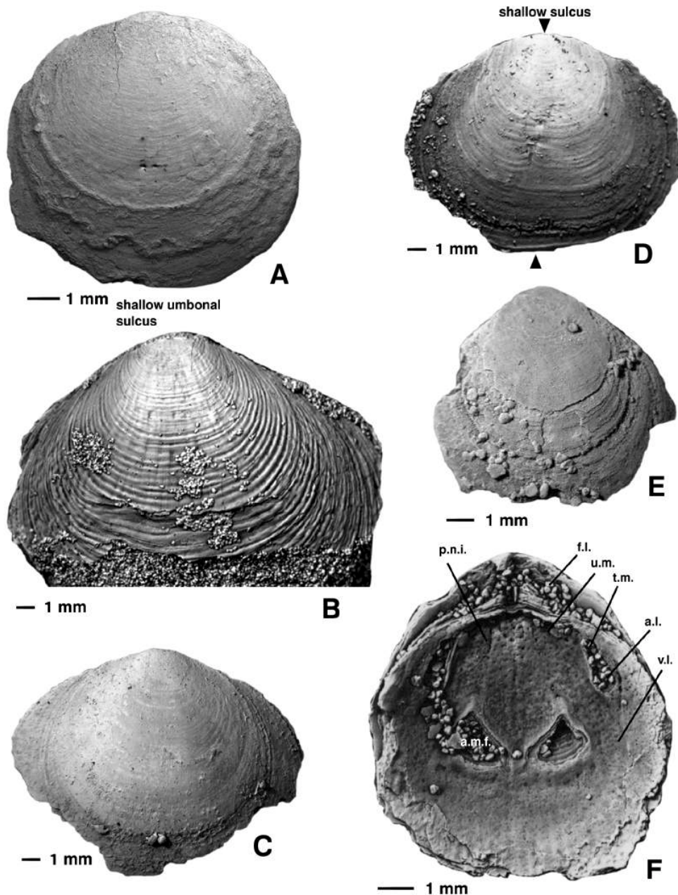
Figure 3: A-E , variations in the external shape of the dorsal valve and ornament in species of Obolus and Ungula . A , Ungula convexa (PANDER, 1830), NMW 2001.39G.4; Upper Cambrian, Ladoga Formation, locality B-2, Unit C 2 (POPOV et alii , 1989, fig. 3), on the right (facing downstream) bank of the Izhora River near the abandoned village of Samsonovka, St Petersburg District; note smooth shell with few growth rings and lack of median sulcus. B , Ungula inomata (MICKWITZ, 1896), CNIGR 160/12348; Upper Cambrian, upper Ulgase Formation, Sample E60/3 (POPOV et alii , 1989, fig. 10), outskirts of the village of Kallavere, North Estonia; note weak umbonal sulcus. C , Obolus transversus (PANDER, 1830), NMW 2001.39G.51; Middle Cambrian, Sablinka Formation, Rebrovo Member, Sample L-41/3 (POPOV et alii , 1989, fig. 2), right-hand side of Volkhov River in southern outskirts of the village of Gorchakovshchina, St Petersburg District; note lack of median sulcus. D , Obolus ruchini KHAZANOVITICH et POPOV, 1984; CNIGR 16/12348; Middle Cambrian, Sablinka Formation, Gertovo Member, Sample L6/1 (POPOV et alii , 1989, fig. 3), right bank of the Sarya River about 700 m downstream from the northern outskirts of the village of Voibokalo; note the very shallow median sulcus, which can be traced in nearly all dorsal valves of Obolus from Gertovo Member. E , Obolus apollinis EICHWALD, 1829; NMW 2001.39G.119; Upper Cambrian, Suurjogi Member, sample 1653/25 (POPOV et alii , 1989, fig. 1), borehole no. 1653 south east of Rakvere, North Estonia; note lack of sulcus. F , View of ventral valve interior of Obolus apollinis EICHWALD, 1829; CNIGR 2/12348; Upper Cambrian, lower Tosna Formation, sample L1/3 (POPOV et alii , 1989, fig. 3), right-hand side of lava River in southern outskirts of the village of Gorodishche; note well developed ventral pseudointerarea with narrow pedicle groove and deep flexure lines (f.l.), pair of weak diverging furrows of pedicle nerve impression (p.n.i.) flanked by paired impression of umbonal muscle scar (u.m.), posterolateral muscle fields bearing attachment scars of transmedian (t.m.) and anterior lateral (a.l.) muscles; paired anterior muscle fields formed by combined attachment scars of central, middle lateral and anterior lateral muscles (a.m.f.) and weakly impressed marginal vascula lateralia (v.l.); depressions under the muscle scars clearly formed as a result of post-mortem degradation of the organic shell matter and subsequent collapse of phosphatic layers.
