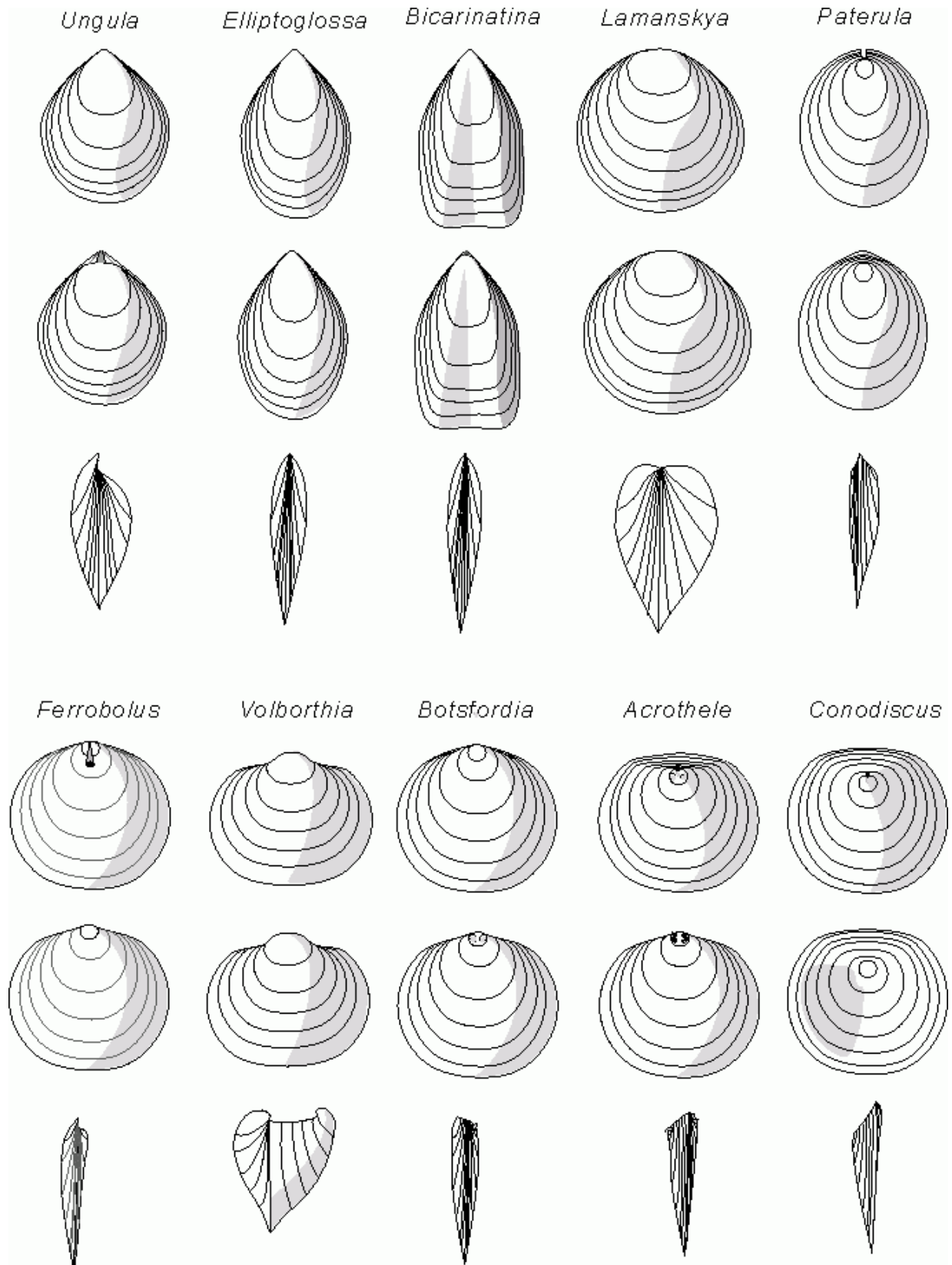
Figure 1: Examples of variations in shell outline and relative valve convexity in selected Palaeozoic lingulide genera.
