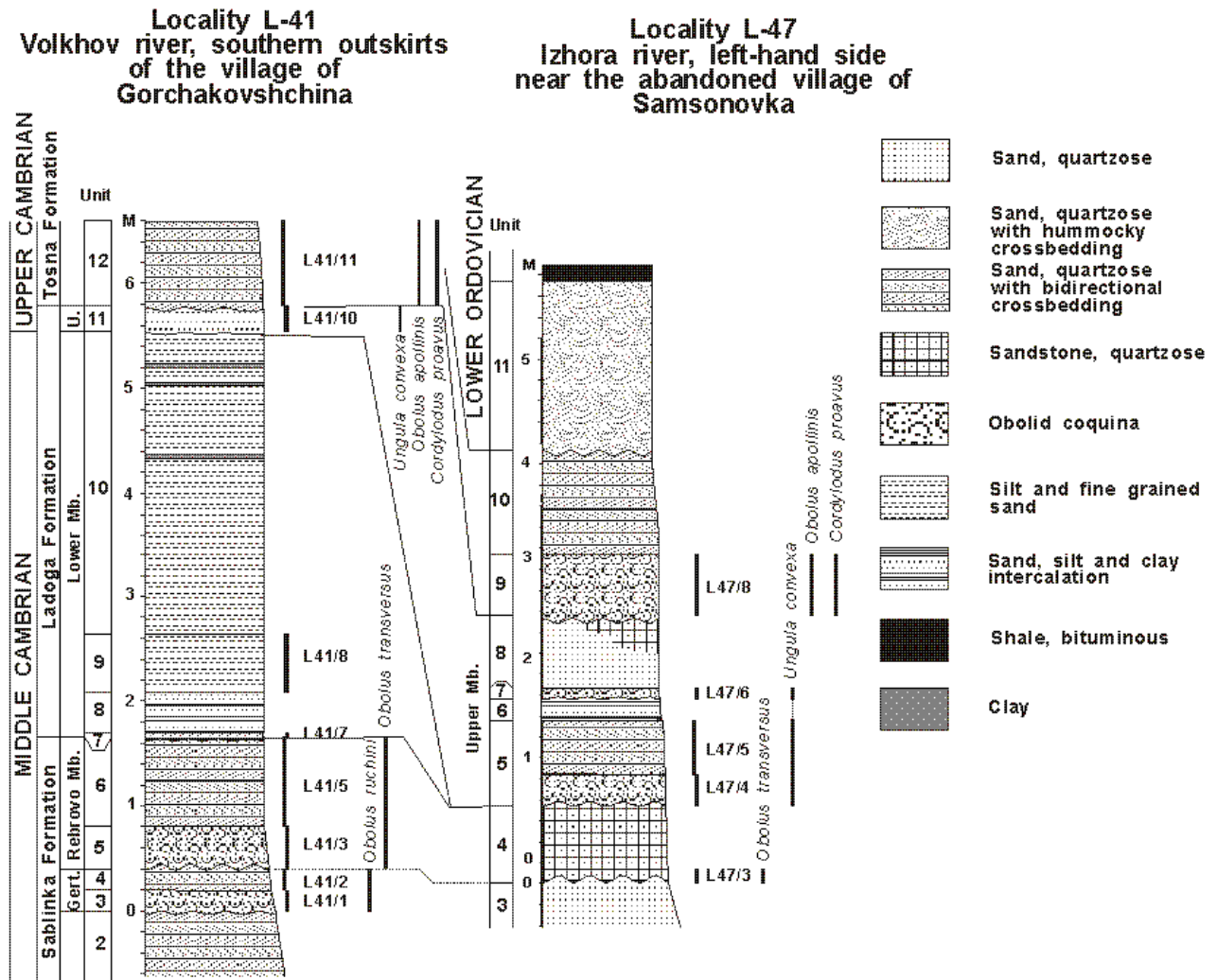
Figure 2: Columnar sections through the Cambrian-Ordovician boundary beds in the East Baltic at the Volkhov and Izhora rivers (see POPOV et alii , 1989, for details) showing of distribution of discussed relevant species.
