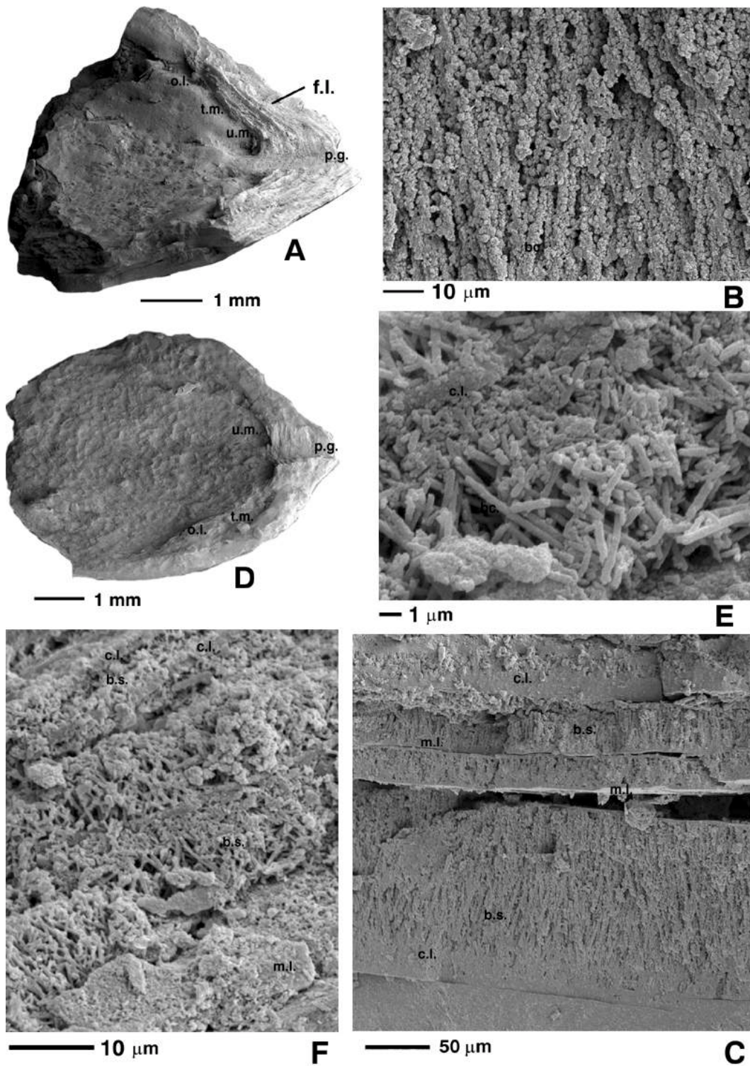
Figure 6: SEM microphotographs of fractured shells of Ungula and Obolus showing basic differences in microstructure under posterolateral muscle fields of the ventral valve (all abbreviations, are the same as on Figs. 3-5, unless otherwise stated). A-C , Ungula convexa (PANDER, 1830), NMW 2001.39G.5, ventral valve; Upper Cambrian, Ladoga Formation, locality B-2, Unit C 2 (POPOV et alii , 1989, fig. 3), right hand side of Izhora River near the abandoned village of Samsonovka, St Petersburg District; A oblique lateral view showing pedicle groove (p.g.) flexure lines and muscle scars; B, symmetrical baculate set showing compactly placed baculi usually exceeding 1 μm in diameter; C, general view through the broken shell showing alternating baculate sets (b.s.), thick compact laminae (c.l.) and membranous laminae (m.l.). D-F , Obolus apollinis EICHWALD, 1829, NMW 2001.39G.109, ventral valve; Upper Cambrian, Tosna Formation, Cordylodus proavus conodont biozone, sample L47/8 (POPOV et alii , 1989, fig. 5), Izhora River, left-hand side, about 800 m upstream of the locality B2; D, oblique lateral view showing pedicle groove, flexure lines and muscle scars; E, general view of baculate set showing relation with compact lamina; F, general view of the shell fracture showing alternating symmetrical baculate sets with loosely spaced inclined baculi and thin compact laminae; note that sizes of major structural elements (e.g. size of baculi and compact laminae) in the Obolus shell are about one order of magnitude smaller than in Ungula .
