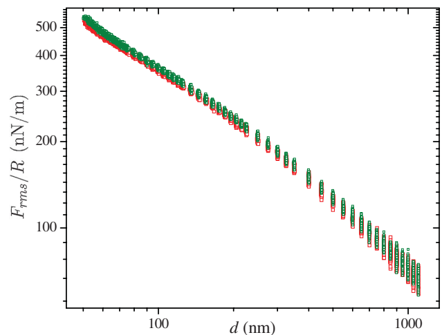
FIG. 3 (color). Hydrodynamic force acting on the sphere as a function of the absolute separation d for Au-Au (green squares) and Au-ITO (red squares), for the data sets shown in Figs. 2(a) and 2(b).
