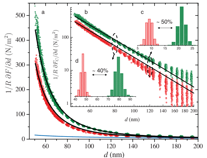
FIG. 2 (color). (a) Spatial derivative of the total force as a function of absolute surface separation for the Au-Au (green squares) and Au-ITO (red squares) interactions for randomly chosen subsets of the data (150 out of 580 for both cases). The blue line represents the derivative of the electrostatic force caused by the simultaneous calibration procedure (common to both the gold and ITO measurements). The black lines indicate the calculated Casimir forces with the electrostatic background added. (b) Spatial derivative of the Casimir force, with the electrostatic background subtracted from the data. The black lines correspond to the calculations of the Casimir force. (c) Histograms of 580 force measurements for Au-Au and Au-ITO at d = 120 nm. (d) Same as c, but for d = 80 nm.
