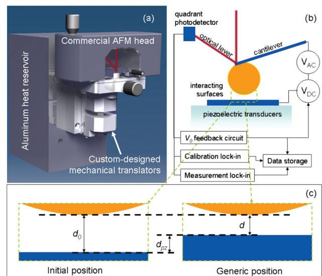
FIG. 1 (color). (a) Drawing of the experimental setup. (b) Schematic representation of the working principle of the experimental technique. (c) Definition of d_0 (initial separation), d_{pz} (movement of the piezoelectric stage), and d (separation between the two surfaces).
