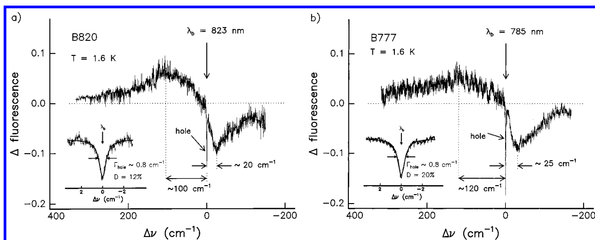
Figure 4. Change of the intensity of the fluorescence excitation spectra after burning a deep hole into B820 (a) and B777 (b) at 1.6 K. The insets show an amplification of the zero-phonon holes. They do not reflect the homogeneous line width due to burning fluence broadening. The phonon side hole is shifted by \sim 20 \text{ cm}^{-1} to the red of the burned hole in B820 and by \sim 25 \text{ cm}^{-1} in B777. The antihole is on the blue side of the burned hole at \sim 100 \text{ cm}^{-1} for B820 and at 120 \text{ cm}^{-1} for B777.
