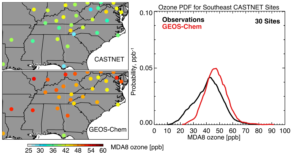
10 Figure 10: Maximum daily 8-h average (MDA8) ozone concentrations at the 30 CASTNET sites in the Southeast US in June-August 2013. The left panels show seasonal mean values in the observations and GEOS-Chem. The right panel shows the probability density functions (pdfs) of daily values at the 30 sites.
