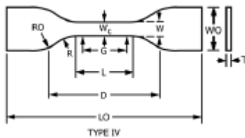
Type IV tensile specimen from ASTM D638
