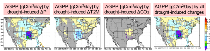
Figure 4: June ΔGPP (local and remote) from isolated and combined contributions of precipitation, temperature, and CO 2 anomalies that are caused by the drought imposed in the Region S. The offline Catchment-CN model was used to isolate the induced changes in the meteorological drivers by the coupled model (from Fig. 3).
