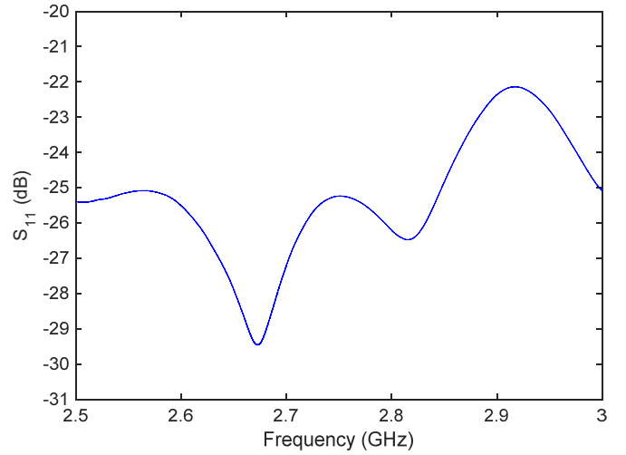
Fig. 3. The EM signature (log magnitude S_{11} response) of the carbon fiber tape from 2.5 GHz to 3 GHz.
