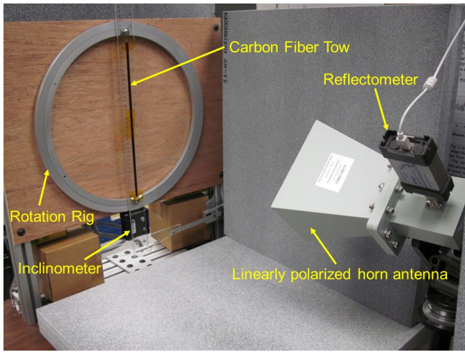
Fig. 2. Experimental setup: carbon fiber tow, tow rotator rig, inclinometer, and linear polarized horn antenna.
