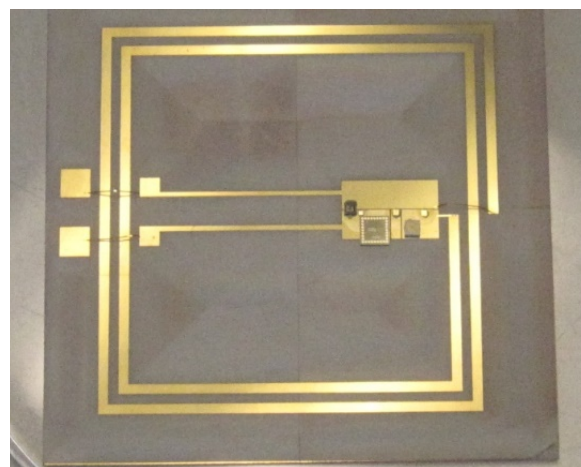
Figure 2: Photograph of pickup coil and rectifying circuit.
