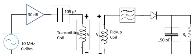
Figure 1: Schematic of inductive power transfer circuit.
