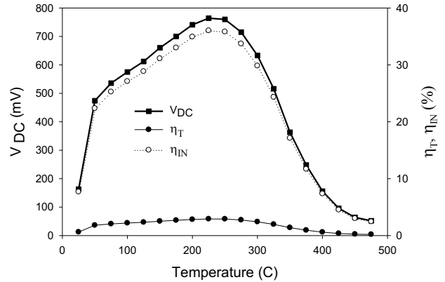
Figure 8: Measured V_{DC} and efficiency.
