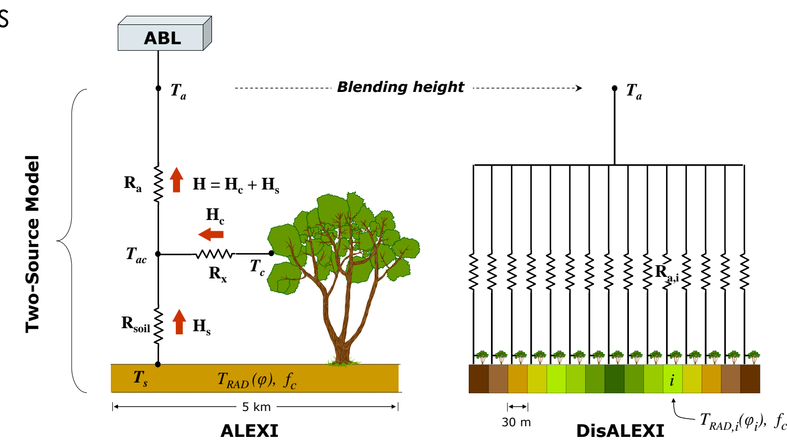
Figure 1. Multi-scale modeling framework: (left) ALEXI system, using morning surface temperature rise from geostationary (GEO) satellites; (right) flux disaggregation using LST from Landsat, MODIS, aircraft, etc.
