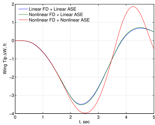
Figure 11. Longitudinal Response of Flexible Wing GTM with 1-Cosine Discrete Gust
