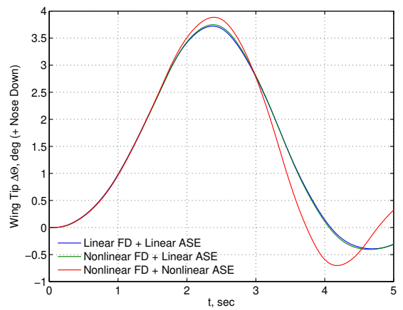
Figure 11. Longitudinal Response of Flexible Wing GTM with 1-Cosine Discrete Gust
