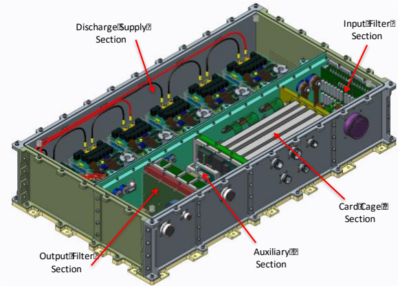
Figure 3: AEPS EDU PPU Design.
