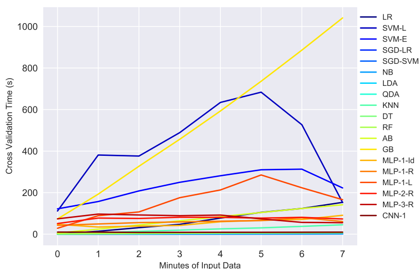
(b) Sensitivity Analysis - Time (s)
