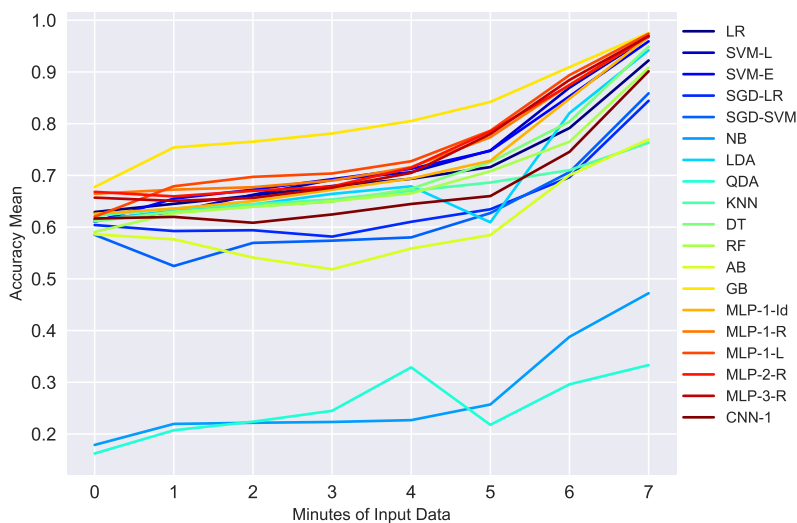
(a) Sensitivity Analysis - Accuracy Mean
