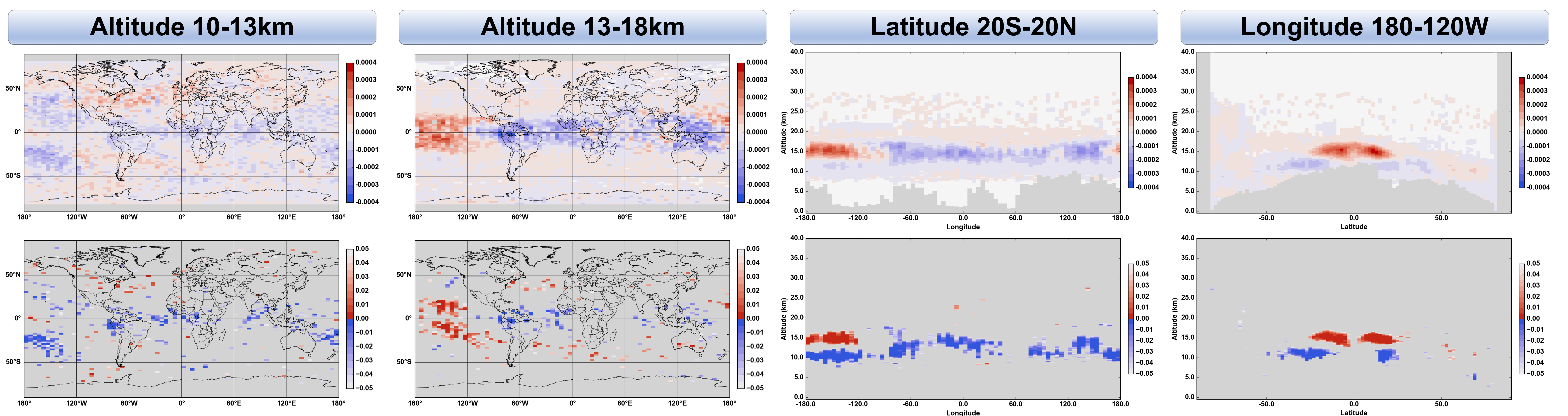
Figure 3: Eastern Pacific Ocean linear regression slopes (top) and p-values (bottom) for monthly average volume occurrence frequencies per bin limiting the z-axis to the values in the labels above the individual plots.
